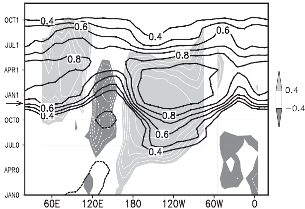
FIG. 5. Longitude–time section of correlation with the NDJ(0) Niño-3.4 index: SST (light shade > 0.4 ; dark < -0.4 ; white contours at intervals of 0.1), and tropospheric temperature (black contours) on the equator. The black arrow denotes December(0), the peak phase of ENSO.
