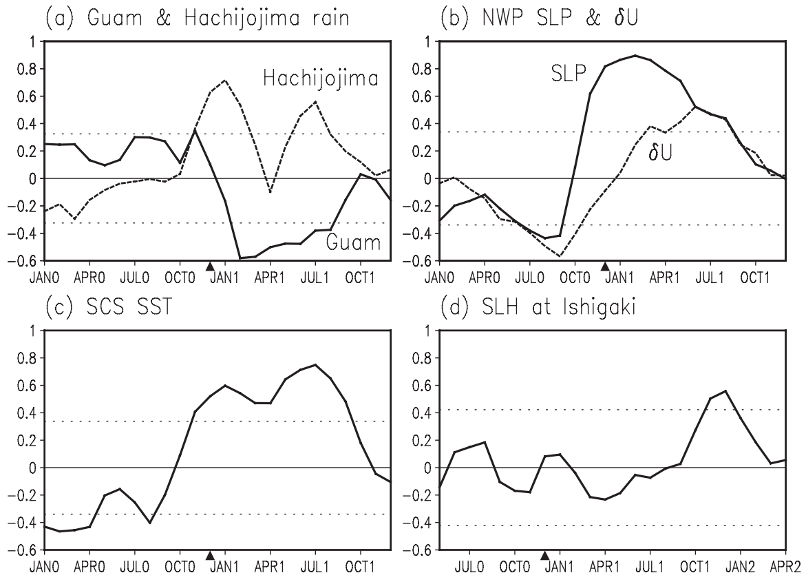
FIG. 2. Correlation with the NDJ(0) Niño-3.4 SST index: (a) rainfall at Guam and Hachio Islands; (b) subtropical NW Pacific SLP ( 10^{\circ} – 25^{\circ} N, 130^{\circ} – 170^{\circ} E), and surface wind vorticity defined as ( 27^{\circ} – 33^{\circ} N) minus ( 11^{\circ} – 15^{\circ} N) zonal wind difference averaged in 120^{\circ} – 150^{\circ} E; (c) SCS SST ( 5^{\circ} – 15^{\circ} N, 110^{\circ} – 125^{\circ} E); and (d) sea level height at Ishigaki Island. (b) and (c) Based on ICOADS. Dotted lines indicate the 95% significance level, which varies with the data record length. (In (a), the significance level is 0.44 for the shorter Hachio record.) The black triangle denotes December(0), the peak phase of ENSO.
