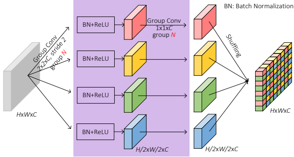
Figure 5: Depthwise index networks. N = C for the O2O assumption, and N = 1 for the M2O. The masked modules are invisible to linear networks.
