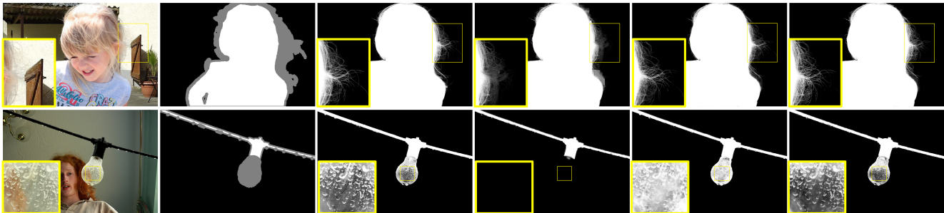
Figure 7: Qualitative results on the Composition-1k testing set. From left to right, the original image, trimap, ground-truth alpha matte, closed-form matting [29], deep image matting [29], and ours (M2O DIN with “nonlinear + context”). See the Supplement for further results.
