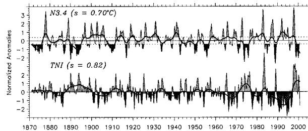
FIG. 1. Time series of SSTs from Niño-3.4 (top), and TNI (bottom) from 1871 to 2000. Both time series are normalized by the standard deviation s , as given. (top) Shading is included to show where thresholds of \pm 0.4^{\circ}\text{C} are exceeded, indicating ENSO events. A low-pass spline fit highlights interdecadal variations.
