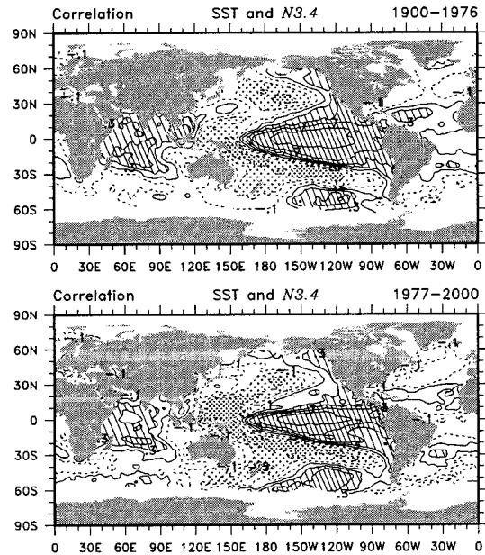
FIG. 3. Correlations of SST anomalies with N3.4 for 1900–76 and 1977–2000. Values exceeding 0.3 are hatched and less than -0.3 are stippled. The contour interval is 0.2.
