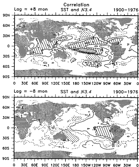
FIG. 5. Correlations of SST anomalies with N3.4 at \pm 8 months lag for 1900–76. Values exceeding 0.3 are hatched and less than -0.3 are stippled. The contour interval is 0.2.
