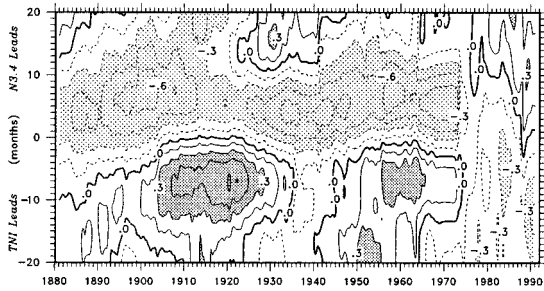
FIG. 2. Moving cross correlations of TNI with N3.4 as 241-month running means (about 20 yr). Negative lag means TNI leads, and positive lag means N3.4 leads. Values exceeding 0.3 in magnitude are shaded.
