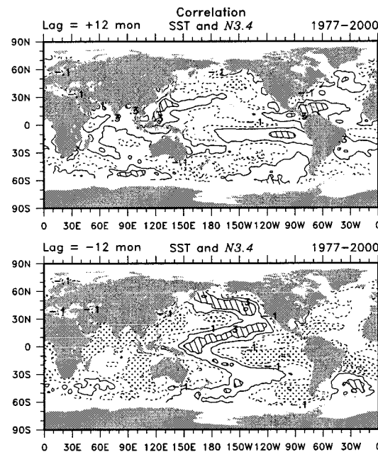
FIG. 6. Correlations of SST anomalies with N3.4 at \pm 12 months lag for 1977–2000. Values exceeding 0.3 are hatched and less than -0.3 are stippled. The contour interval is 0.2.
