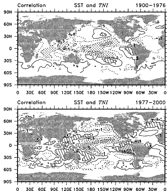
FIG. 4. Correlations of SST anomalies with TNI for 1900–76 and 1977–2000. Values exceeding 0.3 are hatched and less than -0.3 are stippled. The contour interval is 0.2.
