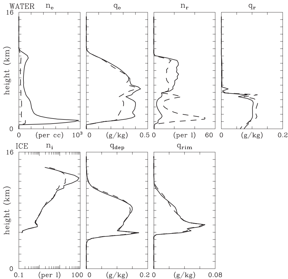
FIG. 6. As in Fig. 5, but for set ST28.
