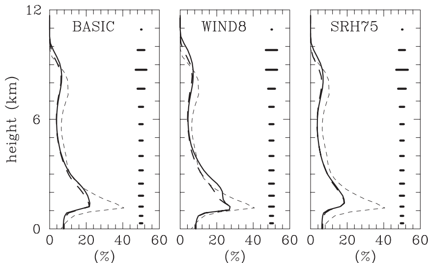
FIG. 4. Quasi-equilibrium profiles of the cloud fraction for simulations POLLUTED (thick solid line) and PRISTINE (thick dashed line) with the homogeneous mixing scenario in BASIC, WIND8, and SRH75. Thin dashed line shows the profile for the PRISTINE homogeneous mixing case of G06. Length of horizontal bars on the right-hand side of each panel represents the averaged standard deviation (i.e., the mean of the POLLUTED and PRISTINE) of the temporal evolution of the domain mean. Bars are shown only at selected levels.
