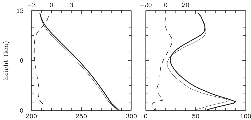
FIG. 3. As in Fig. 2, but comparing profiles for PRISTINE simulations with homogeneous mixing from sets WIND8 (thick line) and SRH75 (thin line). Note the different scales for the SRH75 minus WIND8 differences (shown as dashed lines) when compared to Fig. 2. G06 profiles are not shown.
