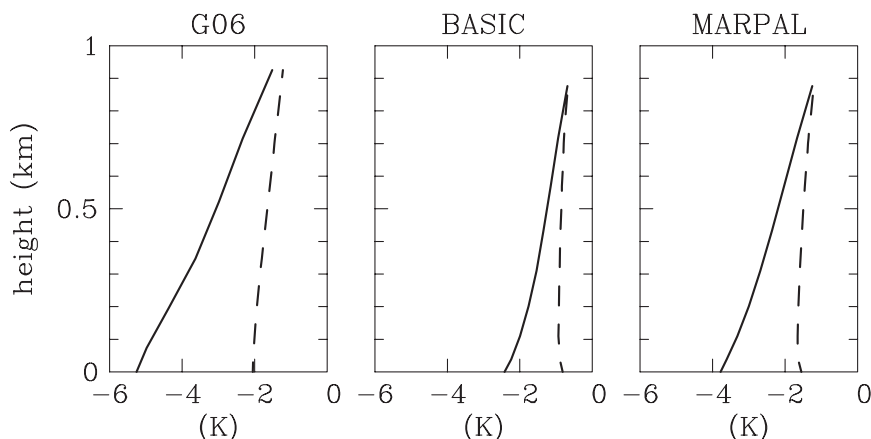
FIG. 7. Potential temperature profiles in the lowest kilometer of the simulation domain shown as deviations from the surface temperature for PRISTINE simulations with the homogeneous mixing discussed in G06 and in similar simulations from the BASIC and MARPAL sets. Solid lines represent profiles sampled over grid points with rain, whereas dashed lines are for domain-averaged profiles.
