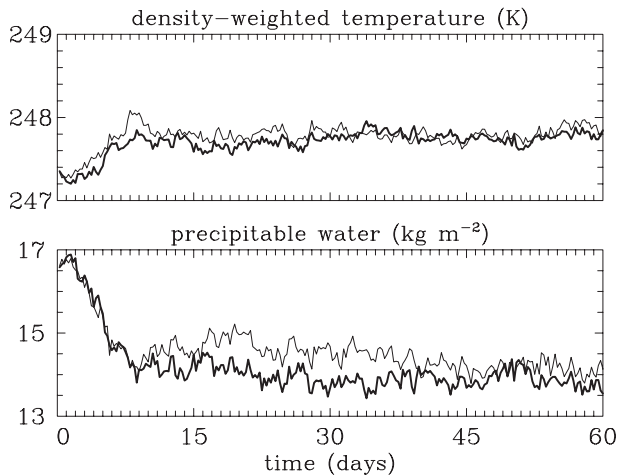
FIG. 1. Evolution of the (top) density-weighted temperature and (bottom) precipitable water for simulations PRISTINE (thick line) and POLLUTED (thin line) with the homogeneous mixing scenario.
