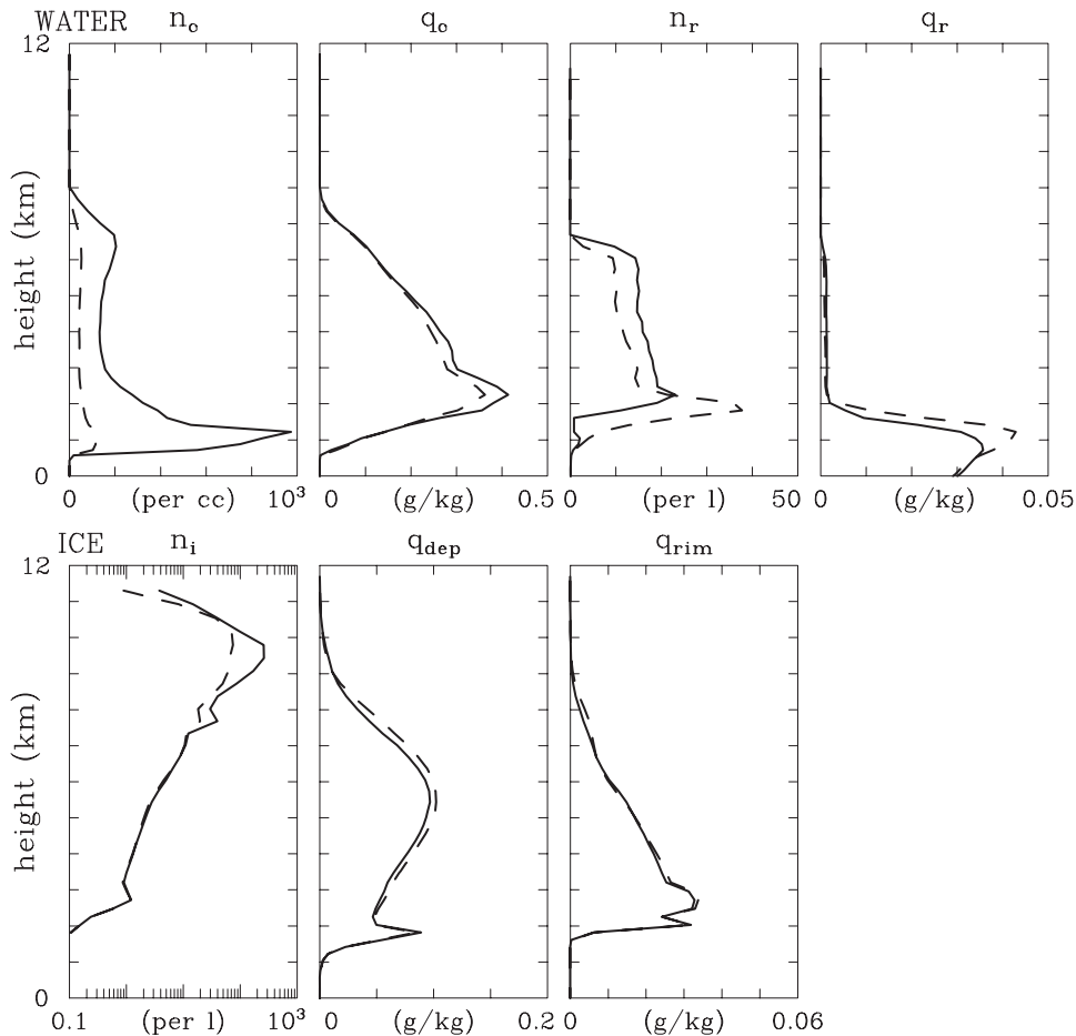
FIG. 5. Quasi-equilibrium profiles of conditionally sampled microphysical fields for POLLUTED (solid line) and PRISTINE (dashed line) BASIC simulations with the homogeneous mixing scenario: (top) water and (bottom) ice. See text for details.
