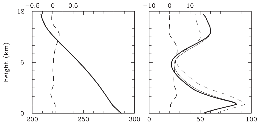
FIG. 2. (left) Quasi-equilibrium temperature and (right) RH profiles for simulations PRISTINE (thick line) and POLLUTED (thin line) with the homogeneous mixing scenario. Initial profiles taken from the simulations discussed in G06 are shown by thin dashed lines (note that the G06 temperature profile is not visible in (left), as all 3 profiles differ less than the thickness of the line). POLLUTED minus PRISTINE differences are shown using the thick dashed lines in the left side of both panels, with the scales provided above each panel.
