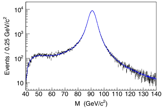
FIG. 7 (color online). Calibrated muon-pair invariant mass distributions over an extended mass range. The crosses are the background-subtracted data and the solid histogram is from the simulation. The comparison of the simulation with the data yields a \chi^2 of 518 for 400 bins.
