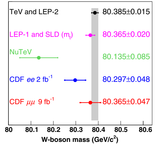
FIG. 18 (color online). Comparison of experimental determinations of the W -boson mass. “TeV and LEP-2” represents direct measurements of the W -boson mass; “LEP-1 and SLD ( m_t )” represents the standard model analysis of Z-pole measurements; “NuTeV” represents the indirect measurement derived from neutrino scattering at Fermilab; “CDF ee \ 2 \text{ fb}^{-1} ” represents the A_4 analysis; and “CDF \mu\mu \ 9 \text{ fb}^{-1} ” represents this analysis. The horizontal bars represent total uncertainties.
