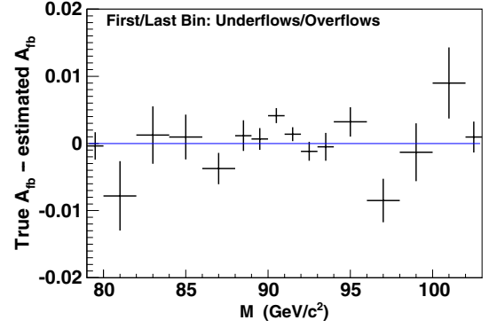
FIG. 14 (color online). Event-weighting bias for each of the muon-pair invariant mass bins. The bias is estimated with the simulation, and the uncertainties represent the full precision of the simulation.
