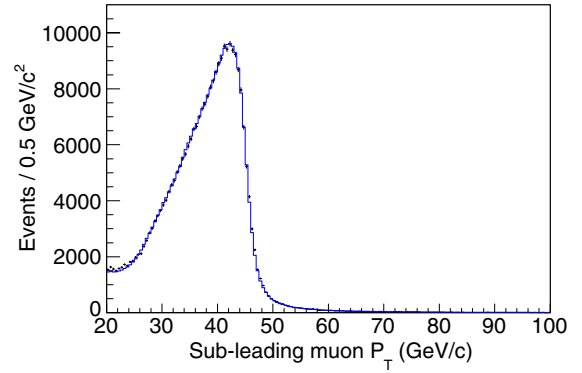
FIG. 9 (color online). Calibrated P_T distribution for the muon with the smaller P_T . The crosses are the background-subtracted data and the solid histogram is from the simulation.
