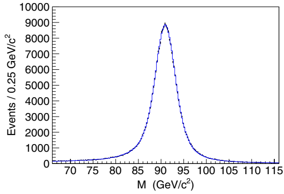
FIG. 6 (color online). Calibrated muon-pair invariant mass distributions. The crosses are the background-subtracted data and the solid histogram is from the simulation. The comparison of the simulation with the data yields a \chi^2 of 219 for 200 bins.
