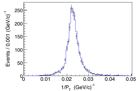
FIG. 4 (color online). Distribution of C^+ for same-side (SS) pairs in the central \eta region of (-0.3, 0) . The crosses are the data, and the solid histogram is the generator-level distribution normalized to the data.
