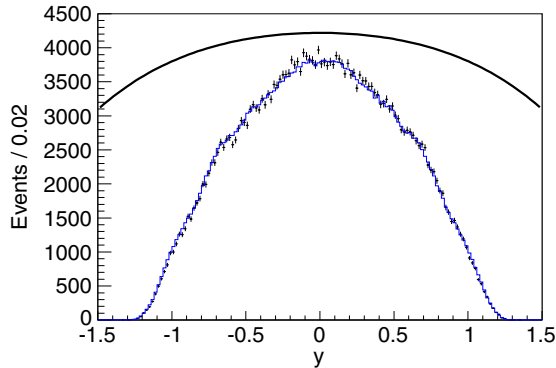
FIG. 13 (color online). Muon-pair y distribution. The crosses are the background-subtracted data and the histogram is the simulation. The measurement is restricted to the region |y| < 1 . The upper curve is the (arbitrarily normalized) shape of the underlying rapidity distribution from PYTHIA.
