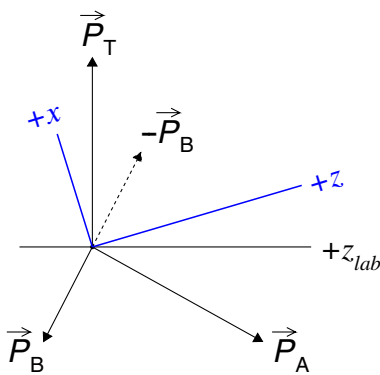
FIG. 1 (color online). CS coordinate axes ( x, z ) in the lepton-pair rest frame, along with the laboratory z axis ( z_{lab} ). The three axes are in the plane formed by the proton ( \vec{P}_A ) and antiproton ( \vec{P}_B ) momentum vectors within the rest frame. Relative to the laboratory z axis, the transverse component of -(\vec{P}_A + \vec{P}_B) is the same as the transverse-momentum vector of the lepton pair in the laboratory ( \vec{P}_T ).
