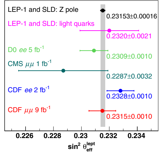
FIG. 17 (color online). Comparison of experimental measurements of \sin^2 \theta_{\text{eff}}^{\text{lept}} . “Z pole” represents the LEP-1 and SLD standard model analysis of Z-pole measurements and “light quarks” represents the LEP-1 and SLD results from the light-quark asymmetries; “D0 ee \ 5 \text{ fb}^{-1} ” represents the D0 A_{\text{FB}}(M) analysis; “CMS \mu\mu \ 1 \text{ fb}^{-1} ” represents the CMS analysis; “CDF ee \ 2 \text{ fb}^{-1} ” represents the A_4 analysis; and “CDF \mu\mu \ 9 \text{ fb}^{-1} ” represents this analysis. The horizontal bars represent total uncertainties.
