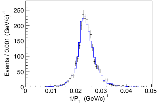
FIG. 5 (color online). Distribution of C^+ for OS pairs in the central \eta region of (-0.3, 0) . The crosses are the data, and the solid histogram is the generator-level distribution normalized to the data.
