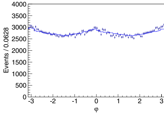
FIG. 11 (color online). Observed \varphi distribution in the Collins-Soper frame. The crosses are the background-subtracted data and the solid histogram is from the simulation.
