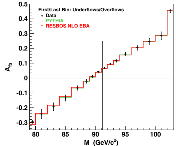
FIG. 15 (color online). Fully corrected A_{fb} . The measurement uncertainties are uncorrelated bin-by-bin unfolding estimates. The vertical line is M = M_Z . The PYTHIA calculation uses \sin^2 \theta_{eff}^{lept} = 0.232 . The EBA-based RESBOS calculation uses \sin^2 \theta_W = 0.2233 ( \sin^2 \theta_{eff}^{lept} = 0.2315 ).
