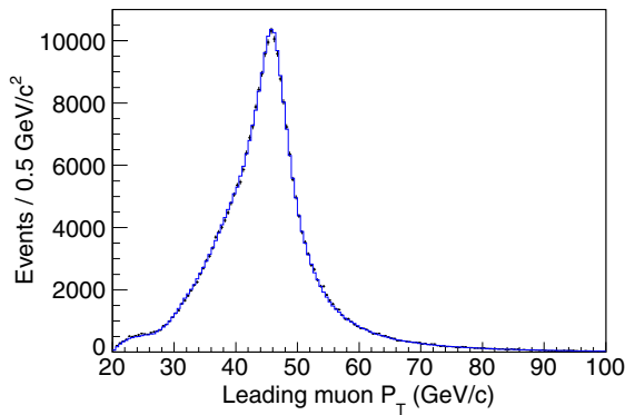
FIG. 8 (color online). Calibrated P_T distribution for the muon with the larger P_T . The crosses are the background-subtracted data and the solid histogram is from the simulation.
