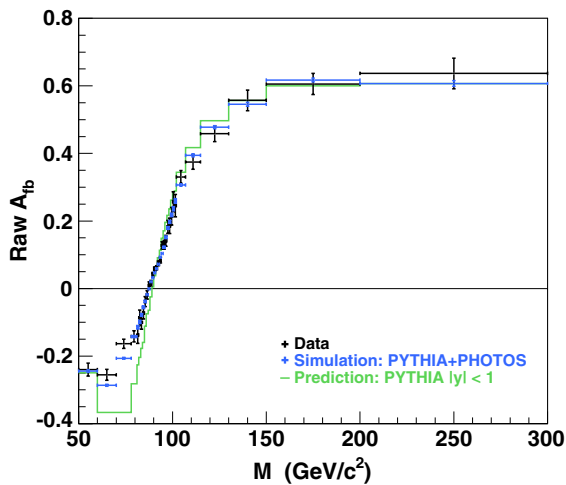
FIG. 12 (color online). Raw A_{\text{fb}} measurement in bins of the muon-pair invariant mass. Only statistical uncertainties are shown. The PYTHIA |y| < 1 asymmetry curve does not include the effect of QED FSR.
