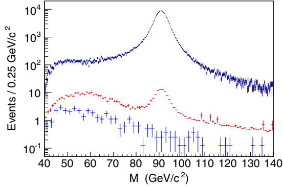
FIG. 2 (color online). Muon-pair invariant mass distributions. The upper set of crosses is the background-subtracted data, the middle set of crosses is the EWK background, and the lower set of crosses is the QCD background (same-charge muon pairs). The EWK background is derived from simulation.
