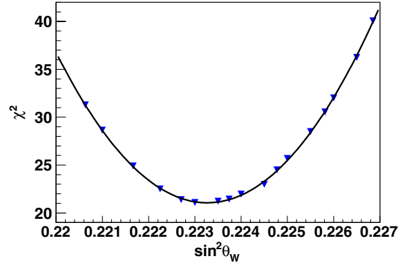
FIG. 16 (color online). Comparison of the A_{\text{fb}} measurement with the RESBOS NLO templates. The triangles are the scan points, and the solid curve is the fit of those points to a generic \chi^2 functional form.
