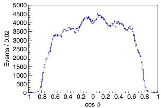
FIG. 10 (color online). Adjusted \cos \vartheta distribution in the Collins-Soper frame. The crosses are the background-subtracted data and the solid histogram is from the simulation.
