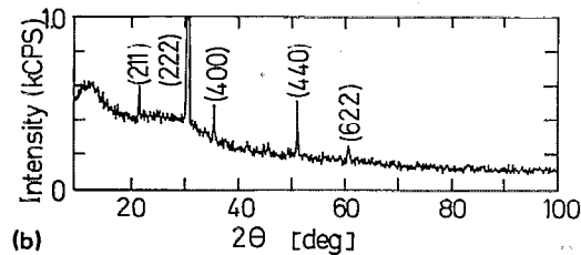
FIG. 2. X-ray diffraction patterns of the (a) 255-nm-thick \text{In}_2\text{O}_3 film and (b) 156-nm-thick \text{In}_2\text{O}_3:\text{Sn} film on borosilicate glass.
