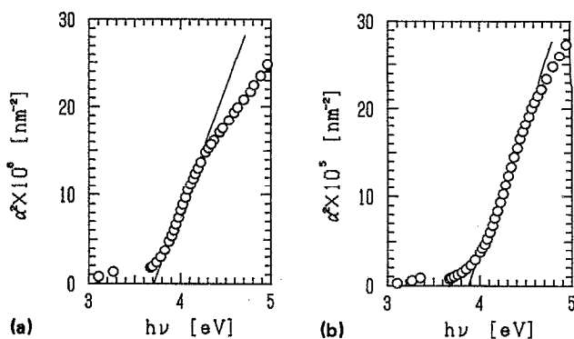
FIG. 6. Square absorption coefficients \alpha^2 for (a) \text{In}_2\text{O}_3 and (b) \text{In}_2\text{O}_3\text{:Sn} ( \text{Sn/In} = 0.01 ) films as a function of photon energy.
