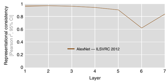
Fig. 6 Representational consistency decreases in AlexNet. We repeated our above analyses of representational consistency on a set of AlexNet instances trained on large-scale object classification data set ILSVRC 2012. Again, we only vary the initial random seed of the network weights. In line with our previous results, we observe a decrease in representational consistency from early to late network layers. The minimal average consistency is observed in layer fc6, which exhibits 62% of the shared variance across network RDMs. As AlexNet requires the input of size 224 × 224, which is significantly larger than the 32 × 32 image size of CIFAR-10 used earlier, we created an independent set of larger images from the same 10 categories while following the same data set structure (100 images per CIFAR-10 category). Ten network instances correspond to 45 pairwise distance estimates per network layer, average representational consistency shown here with 95% confidence intervals (bootstrapped).
