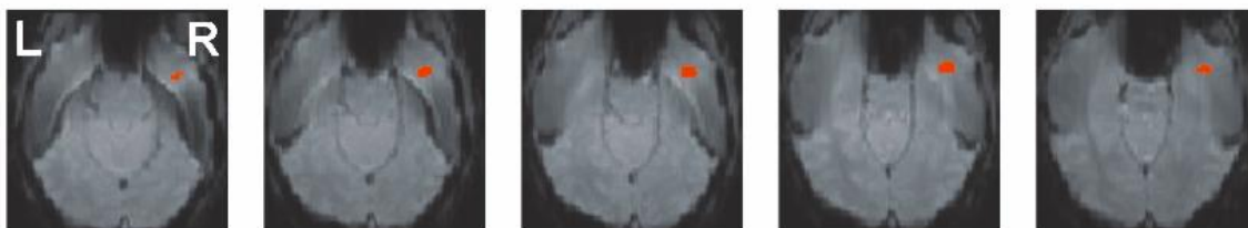
Fig. 11. Anterior inferotemporal face-exemplar region (subject TS). (a) Event-related spatial response patterns elicited by the four images in the anterior temporal face-exemplar region of subject TS. The face-exemplar effect, but none of the other pairwise effects, is significant in this subject. The two horizontal dimensions of each surface plot represent an approximate local cortical flatmap obtained by a neighborhood-preserving projection of the voxels onto the unit square. The vertical axes represent single-image beta estimates. Each voxel is represented by a little black circle and the pattern is interpolated to yield a smooth surface. For an explanation of the central pairwise-effects icon, see legend of SI Fig. 10. The region was defined based on data set A using information-based brain mapping (see Methods ). Data set B was used (i) to compute the event-related spatial response patterns, (ii) to estimate single-trial pairwise condition information (numbers on central pairwise-effects icon; 0 for effects of inconsistent direction between data set A and data set B), and (iii) to test the effect (red connection indicates P < 0.01 in data-set-B t test on a linear discriminant defined by data set A). The spatial-mean effects have been removed by subtracting the spatial-mean time course of the region from each single-voxel time course before the analysis. (Omitting this step yields the same pattern of multivariate effects with negligible changes to the effect sizes.) (b) The anatomical location of the face-exemplar region in subject TS. The anatomical background slices were obtained by averaging the functional volumes across time. Slices progress from inferior to superior (left to right).
