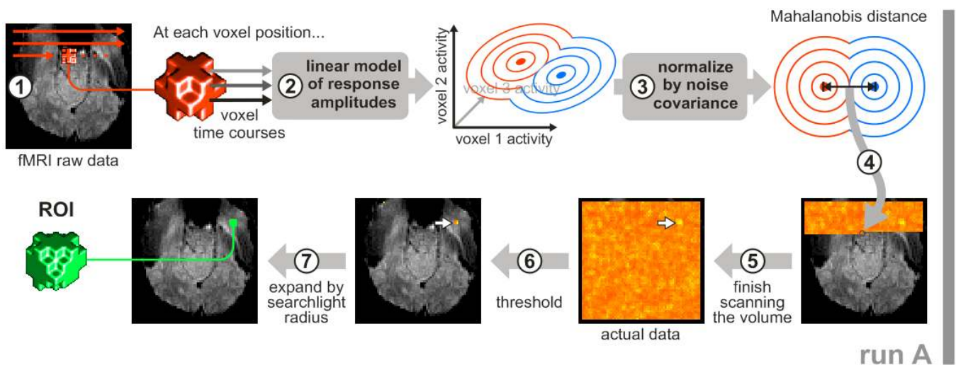
Fig. 8. Information-based response-pattern analysis. (a) For a region of interest (ROI, green voxel cluster) predefined by statistical mapping (1), a linear-model fit (2) provides an estimate of the response amplitude during each condition for each voxel of the region. For each condition, the pattern of responses across the voxels of the ROI can be thought of either as a point in the multidimensional space spanned by the voxel activities (3, red and blue central dots) or as an event-related spatial response pattern on the cortex (4). The analysis is applied to each pair of conditions in turn and is illustrated only for the face pair. For visualization of the ROI's response patterns, we compute an approximation to a regional cortical flatmap by a neighborhood-preserving self-organizing projection of the 3D voxel locations onto the unit square. The response patterns shown (4) are those found in the
