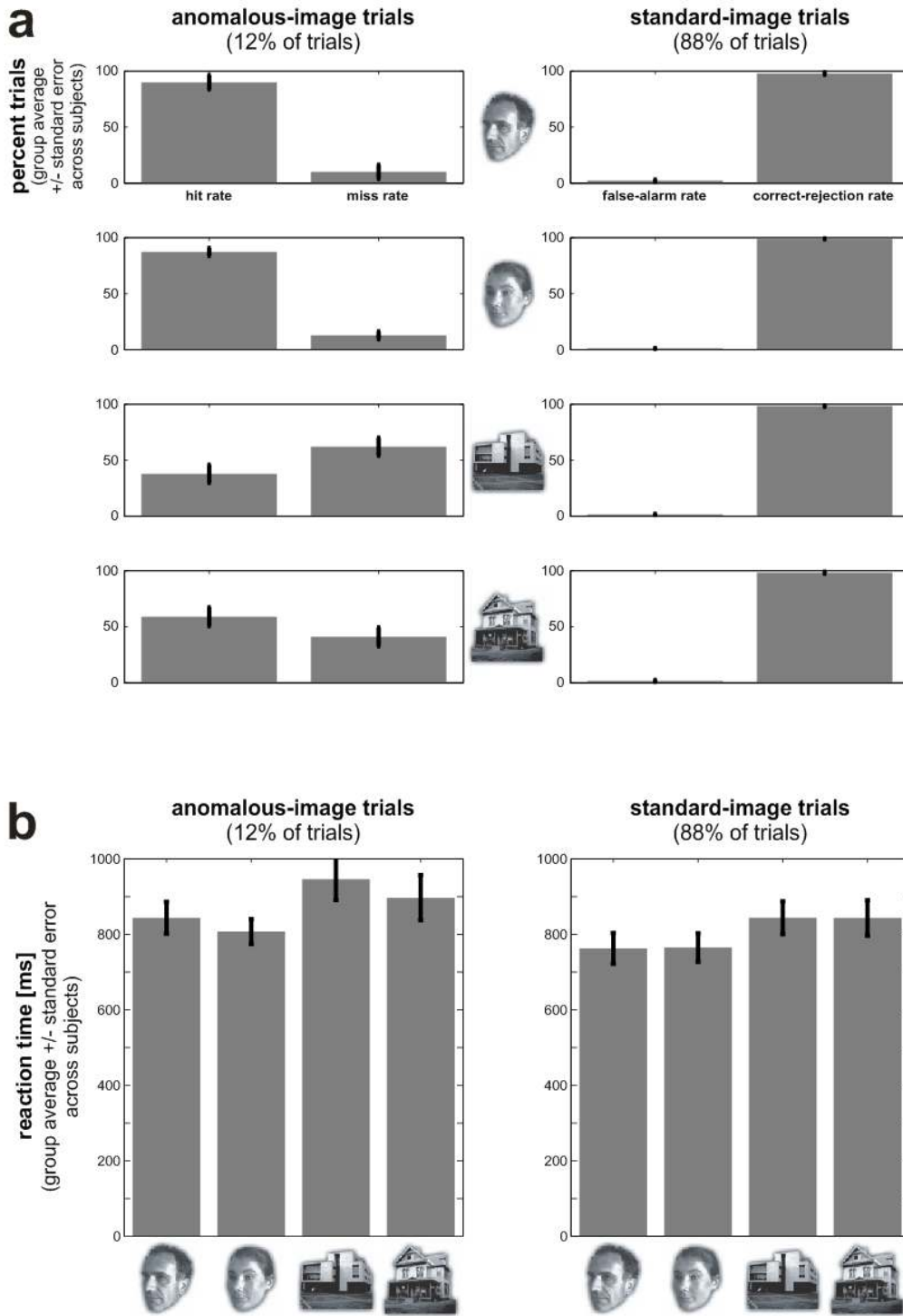
Fig. 5. Detailed behavioral results for anomaly-detection task during fMRI (stimulus-specific reaction times and error rates). (a) Anomaly-detection error analysis as in SI Fig. 10, but performed separately for each of the four standard images (right column) and its anomalous variants (left column). Subjects performed similarly on each of the four standard images. (Only standard-image trials were used for the fMRI analyses.) However, they missed more anomalies for the houses than for the faces. (b) Reaction-time analysis for each of the four standard images (right column) and its anomalous variants (left column). Both error rates and reaction times indicate that the anomaly detection task was slightly more challenging to subjects for the houses than for the faces. Bars show group-average percentages of trials (a) and reaction times (b) with error bars in both indicating the standard error of the mean (computed from the standard deviation of the single-subject means).
