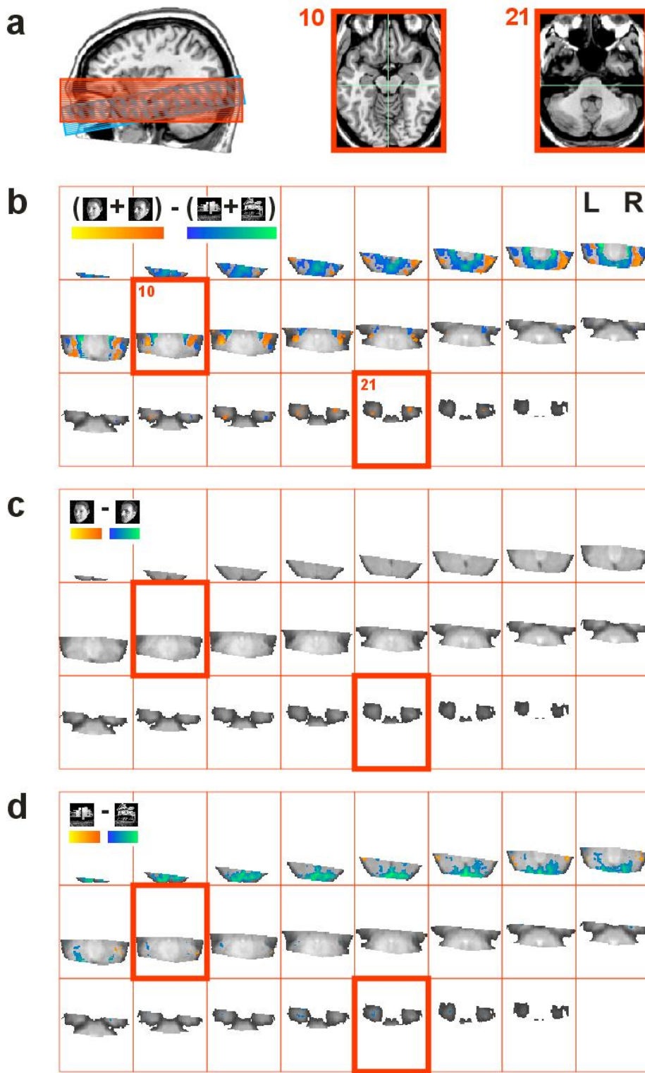
Fig. 7. Activation-based group mapping in Talairach space. (a)
