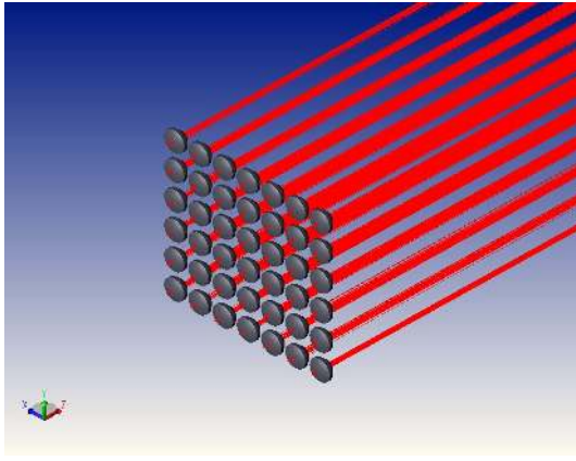
Fig. 15. Non-sequential components shaded model of the array of 7 \times 6 laser diodes and lenses.
