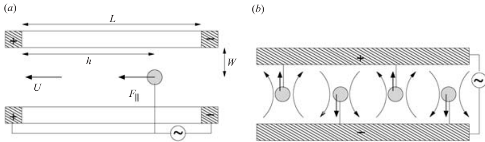
FIGURE 7. Fixed-potential ICEO pumps (a) and mixers (b) can be constructed by electrically coupling the ‘inducing conductor’, which may be a post (as shown) or a surface pattern (not shown), to one set of electrodes. These devices generalize ‘AC electro-osmosis’ in flat-surface electrodes arrays to other situations, with different flow patterns and frequency responses.
