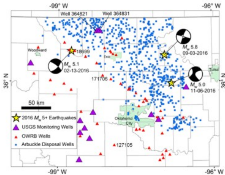
▲ Figure 1. Locations of the epicenters (yellow stars) and focal mechanism of three 2016 M_w \geq 5 earthquakes in Oklahoma; smaller earthquakes are not plotted in order not to clutter the diagram. The locations of U.S. Geological Survey (USGS) wells (large triangles) and Oklahoma Water Resource Board (OWRB) wells (small triangles) are also plotted. The responding wells are labeled with identification numbers. Injection wells operating in the Arbuckle formation, which dispose waste fluid from oil and gas production, are shown with squares. The color version of this figure is available only in the electronic edition.
