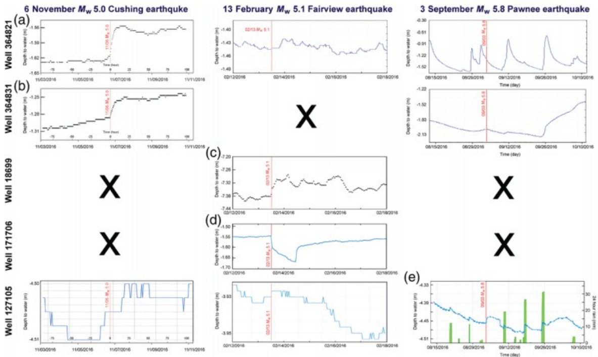
▲ Figure 2. Water level in five wells before and after the three M_w > 5.0 earthquakes in Oklahoma in 2016. Bold X indicates cases with no data; vertical lines show the time of the earthquakes. For clarity, only panels with coseismic changes of water level that are also discussed are labeled. (a) Coseismic change of water level in USGS well 364821 during the 6 November M_w 5.0 Cushing earthquake. (b) Coseismic change of water level in USGS well 364831 during the 6 November M_w 5.0 Cushing earthquake. (c) Coseismic change of water level in OWRB well 18699 before and after the 13 February M_w 5.1 earthquake. (d) Coseismic change of water level in OWRB well 171706 before and after the 13 February M_w 5.1 earthquake. (e) Coseismic change of water level in OWRB well 127105 (blue curve) before and after the 3 September M_w 5.8 Pawnee earthquake. Daily precipitation is shown in vertical bars. The color version of this figure is available only in the electronic edition.
