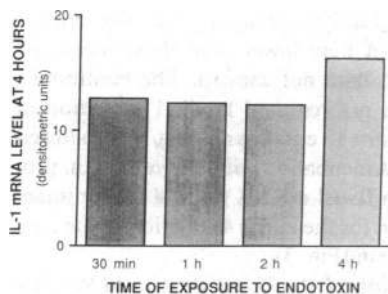
Figure 3. Maximal induction of IL-1 \beta mRNA in SMCs does not require continued presence of endotoxin. Human saphenous vein SMCs were incubated with or without endotoxin ( E. coli ; 055:B5, 1 \mu g/ml). After exposure to endotoxin for the times indicated, the cells
