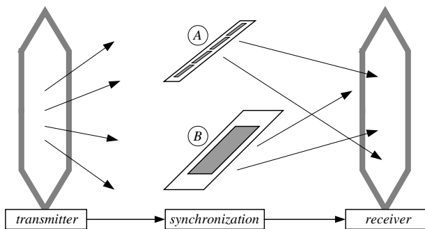
Fig. 40. Magnetic article surveillance system: A) magnetic harmonic system, B) magneto-acoustic system
