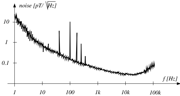
Fig. 7. An example of the noise performance of the induction magnetometer (after [26])
