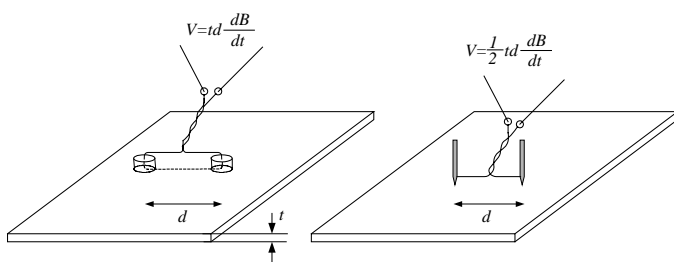
Fig.32. Two methods of local flux density measurements : micro-holes method and needle method
