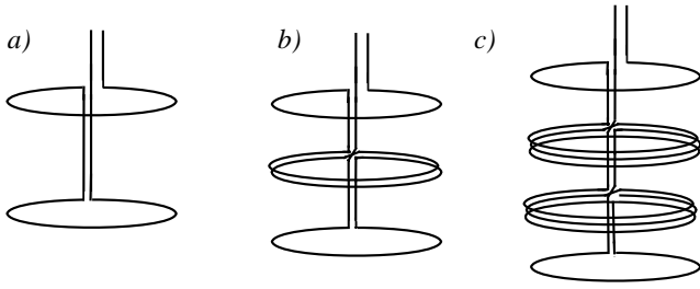
Fig. 23. Gradiometers of a) first-order, b) second-order, c) third-order
