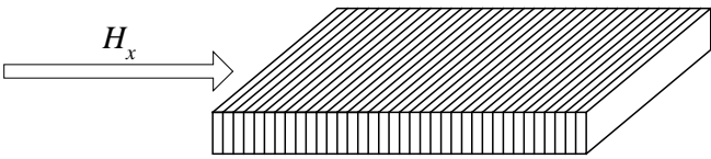
Fig.30. An example of a typical H-coil sensor
