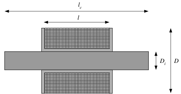
Fig.5. Design of a typical ferromagnetic core coil sensor ( l – length of the coil, l_c – length of the core, D – diameter of the coil, D_i – diameter of the core)
