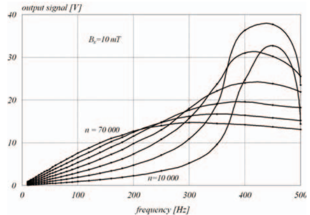
Fig. 36. Frequency characteristics of the constructed sensor
