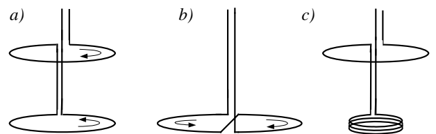
Fig.22. Gradiometer coils arranged: a) vertically, b) horizontally, c) asymmetrically
