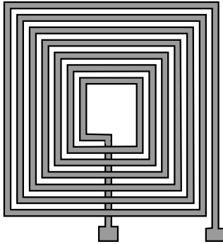
Fig. 4. An example of a pickup planar thin film coil designed for eddy-current sensors [20]
