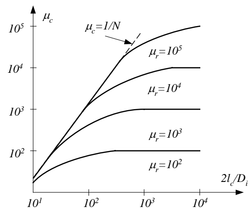
Fig.6. The dependence of the resultant permeability of the core on the dimensions of the core and the permeability of the material [13]
