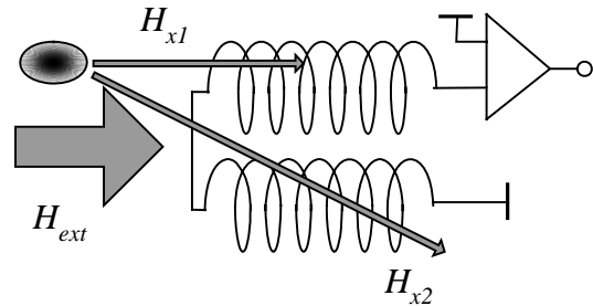
Fig. 21. Operating principle of gradiometer sensor
