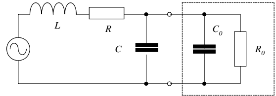
Fig. 9. Equivalent circuit of induction sensor loaded with capacity C_0 and resistance R_0
