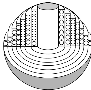
Fig.29. An example of the spherical coil sensor
