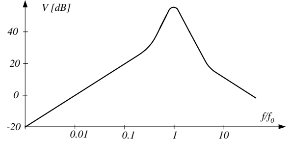
Fig.8. Typical frequency characteristic of an induction coil sensor
