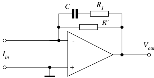
Fig.14. Current to voltage transducer with additional frequency correction circuit. An example described in [26] with elements: R_1 = 100\text{ k}\Omega , C = 0.22\text{ }\mu\text{F} , R' = 47\text{ M}\Omega .
