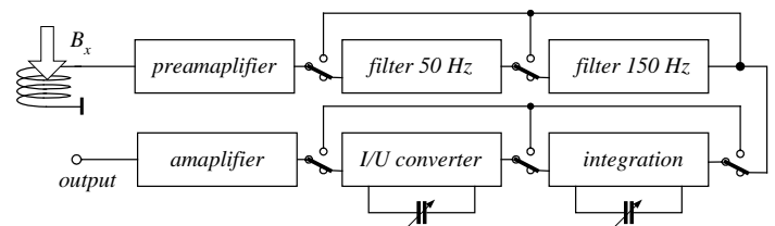
Fig. 37. Block diagram of the induction magnetometer
