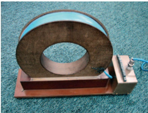
Fig. 35. The air coil sensor designed for investigations of magnetic pollution
