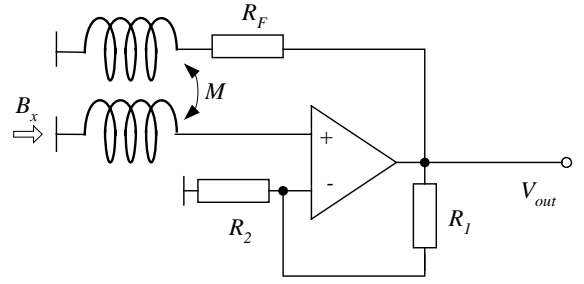
Fig.11. Induction coil sensor connected to the amplifier with negative transformer type feedback
