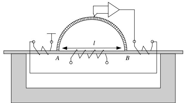
Fig. 26. The application of Rogowski coil for determination of H \cdot l value
