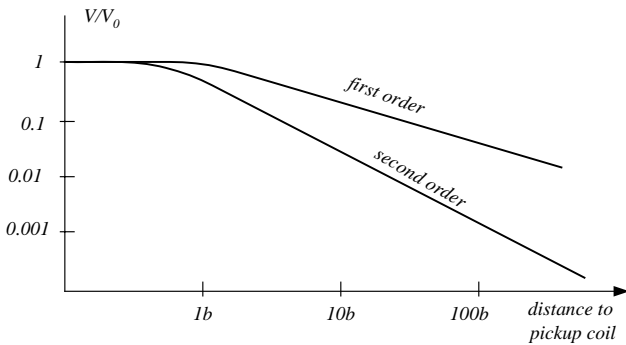
Fig. 24. A typical response of a gradient coil sensor to the source distanced from the pickup coil – relative to response for the source with distance smaller than 0.3b ( b the distance between coils of gradiometer) (after [50])
