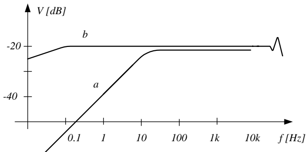
Fig. 15. Frequency characteristic of a coil sensor with current-to-voltage transducer (a) and with additional correction circuit (b)
