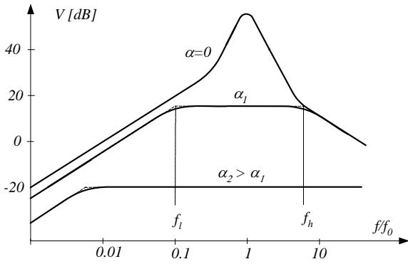
Fig. 10. Frequency characteristics of the induction coil loaded by the resistance R_0 (the coefficient \alpha = R/R_0 )
