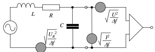
Fig. 18. The sources of the noise in the equivalent circuit of the coil connected to amplifier
