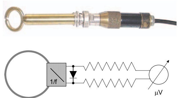
Fig. 38. magnetic field sensor for the frequency bandwidth 0.6 - 2 GHz.
