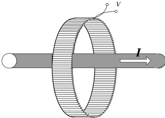
Fig.27. The Rogowski coil as the current I sensor
