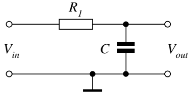
Fig. 13. The passive integrating circuit
