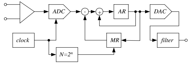
Fig.16. Digital transducer of the coil sensor signal (after [43])
