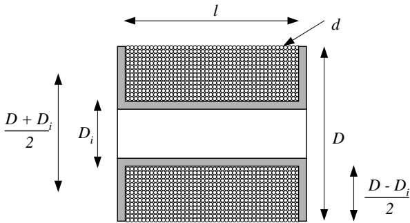
Fig.2. Typical design of an air coil sensor ( l – length of the coil, D – diameter of the coil, D_i – internal diameter of the coil, d – diameter of the wire)
