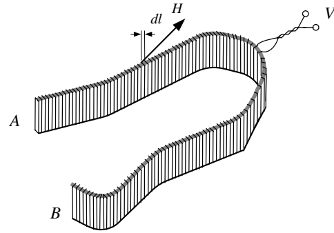
Fig. 25. An example of the Rogowski coil (A, B – ends of the coil)
