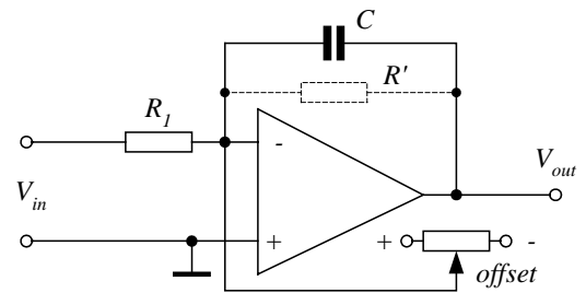
Fig.12. Typical integrating circuit for the coil signal
