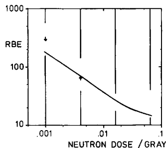
TEXT-FIGURE 11.—Dependence of the RBE of neutrons for the induction of mammary neoplasms on neutron dose. Vertical bars indicate the ranges of RBE that are excluded on a level of statistical significance exceeding 95%; arrows represent differences with lower level of significance. This analysis utilizes a nonparametric method (23) and is based on the current results and on earlier data (7) for gamma rays. The graph applies equally whether one considers FA only or both types of neoplasms.
