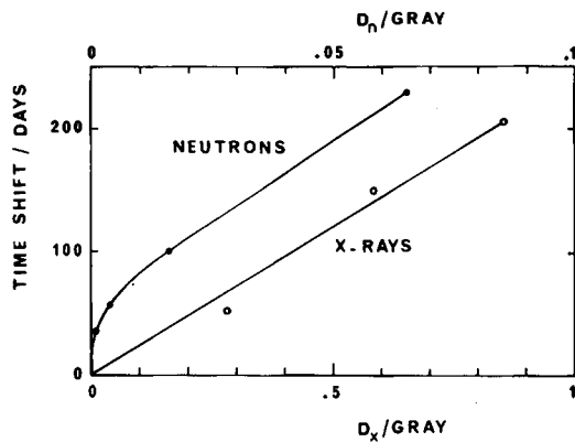
TEXT-FIGURE 10.—Forward shift in time of occurrence of FA due to neutron or X-ray exposure. Scales for the neutron dose ( D_n ) and the X-ray dose ( D_x ) differ by a factor of 10. Time shifts are obtained from the data in text-fig. 4.
