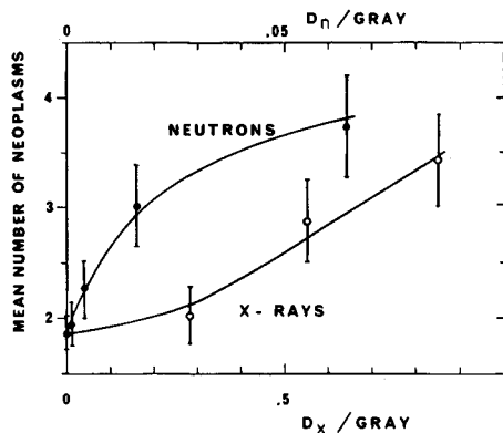
TEXT-FIGURE 1.—Mean No. of mammary neoplasms of any type, FA and AC, throughout life per animal as a function of neutron dose ( D_n ) and X-ray dose ( D_x ). Scales for the neutron dose and the X-ray dose differ by a factor of 10.
