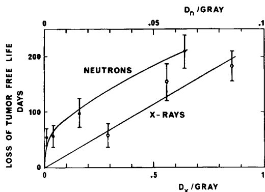
TEXT-FIGURE 2.—Loss of tumor-free life in days for any type of mammary neoplasm, FA, and/or AC as a function of neutron dose ( D_n ) and X-ray dose ( D_x ). Scales for the neutron dose and the X-ray dose differ by a factor of 10.
