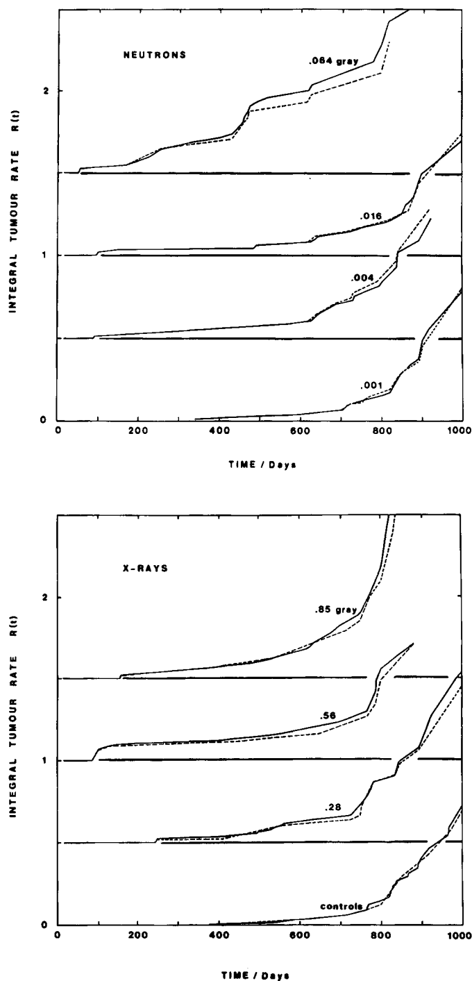
TEXT-FIGURE 7.—Comparison of integral tumor rates R(t) for AC from computations based on all AC (solid lines) and on first AC only (broken lines). Vertical shifts of the curves are as in text-fig. 6.
