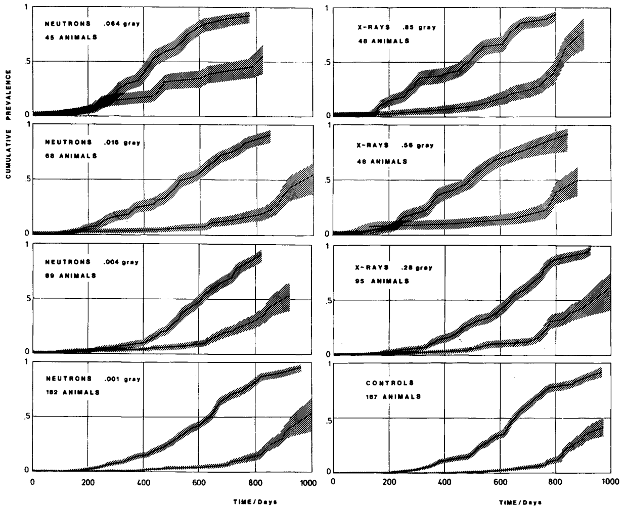
TEXT-FIGURE 8.—Cumulative prevalence I(t) as a function of time after exposure to neutrons or X-rays. In each panel, the curves for FA and AC are given separately; shaded areas represent the SE's.
