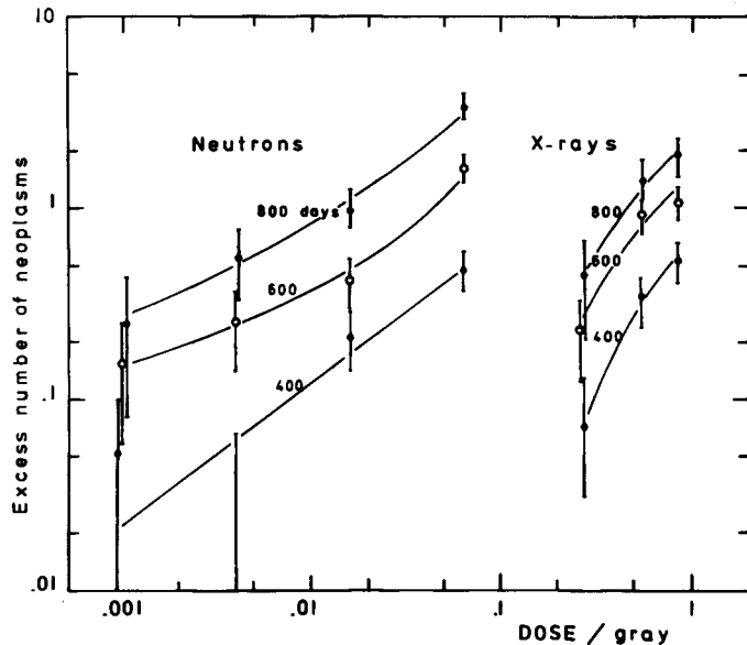
TEXT-FIGURE 9.—Excess No. of FA per animal at specified times after exposure to 430-keV neutrons or X-rays. Data correspond to those in text-fig. 4. Bars are SE's. Solid lines have no mathematical significance; they are inserted merely to clarify the representation.
