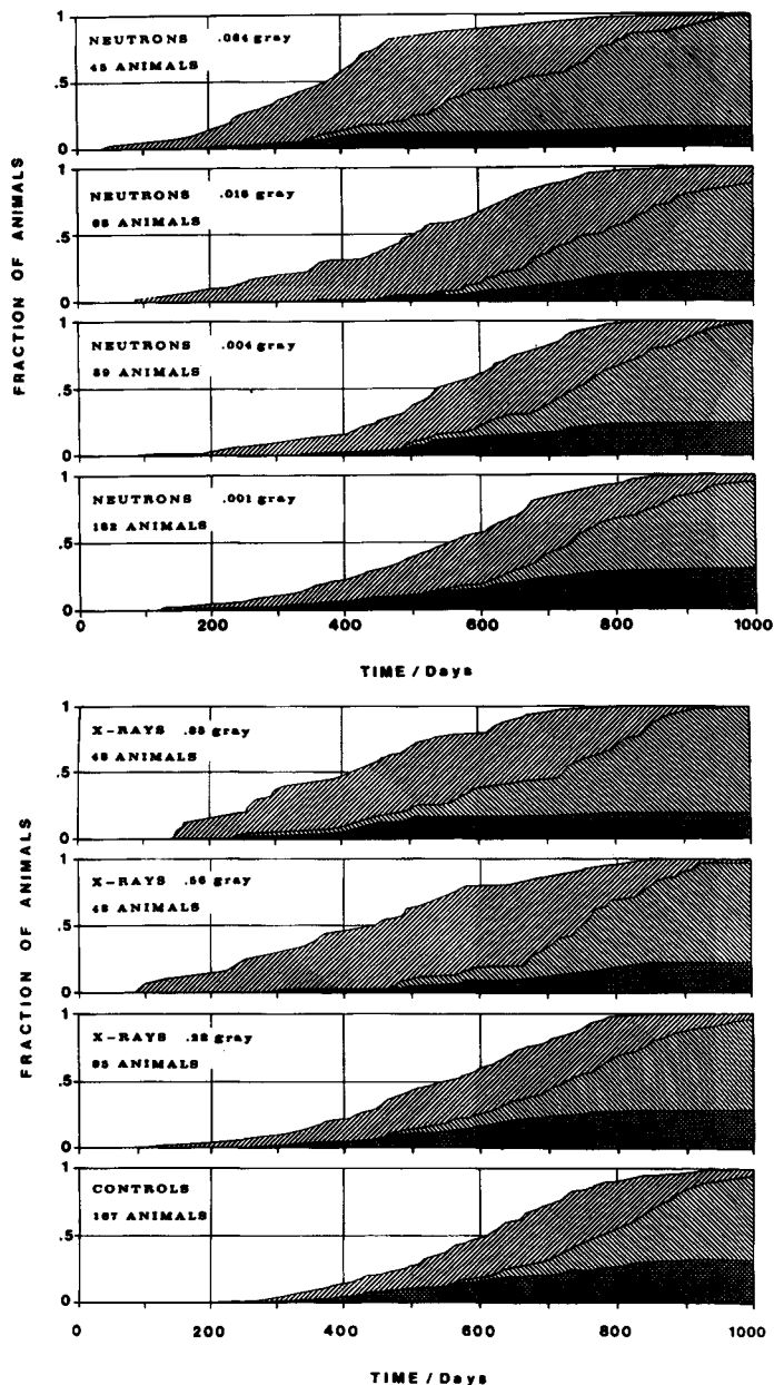
TEXT-FIGURE 3.—Fraction of animals dead or alive with and without a mammary neoplasm of any type, either FA and/or AC, as a function of time after irradiation. ■, Fraction of animals dead without tumor; ▨, fraction of animals dead with at least 1 tumor; ▩, fraction of animals alive with at least 1 tumor; □, fraction of animals alive without tumor.
