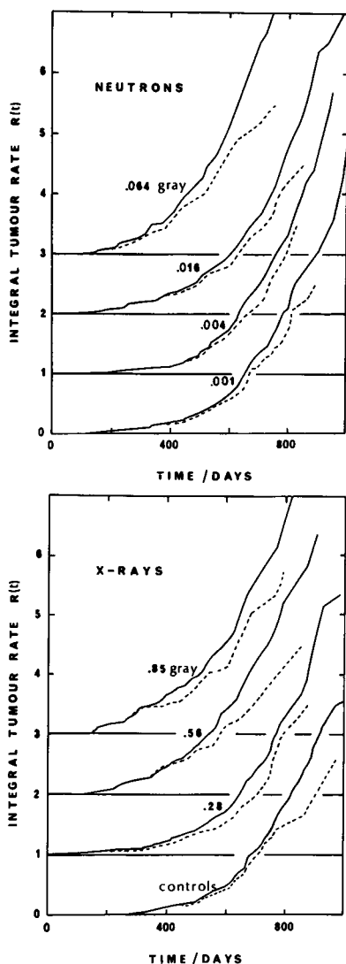
TEXT-FIGURE 6.—Comparison of integral tumor rates R(t) for FA from computations based on all FA (solid lines) and on first FA only (broken lines). To avoid overlap, different shifts of the ordinate values are applied to the curves. The numerical values on the ordinate apply, therefore, only to the unshifted pairs of curves. For the other curves, the ordinate values must be adjusted.
