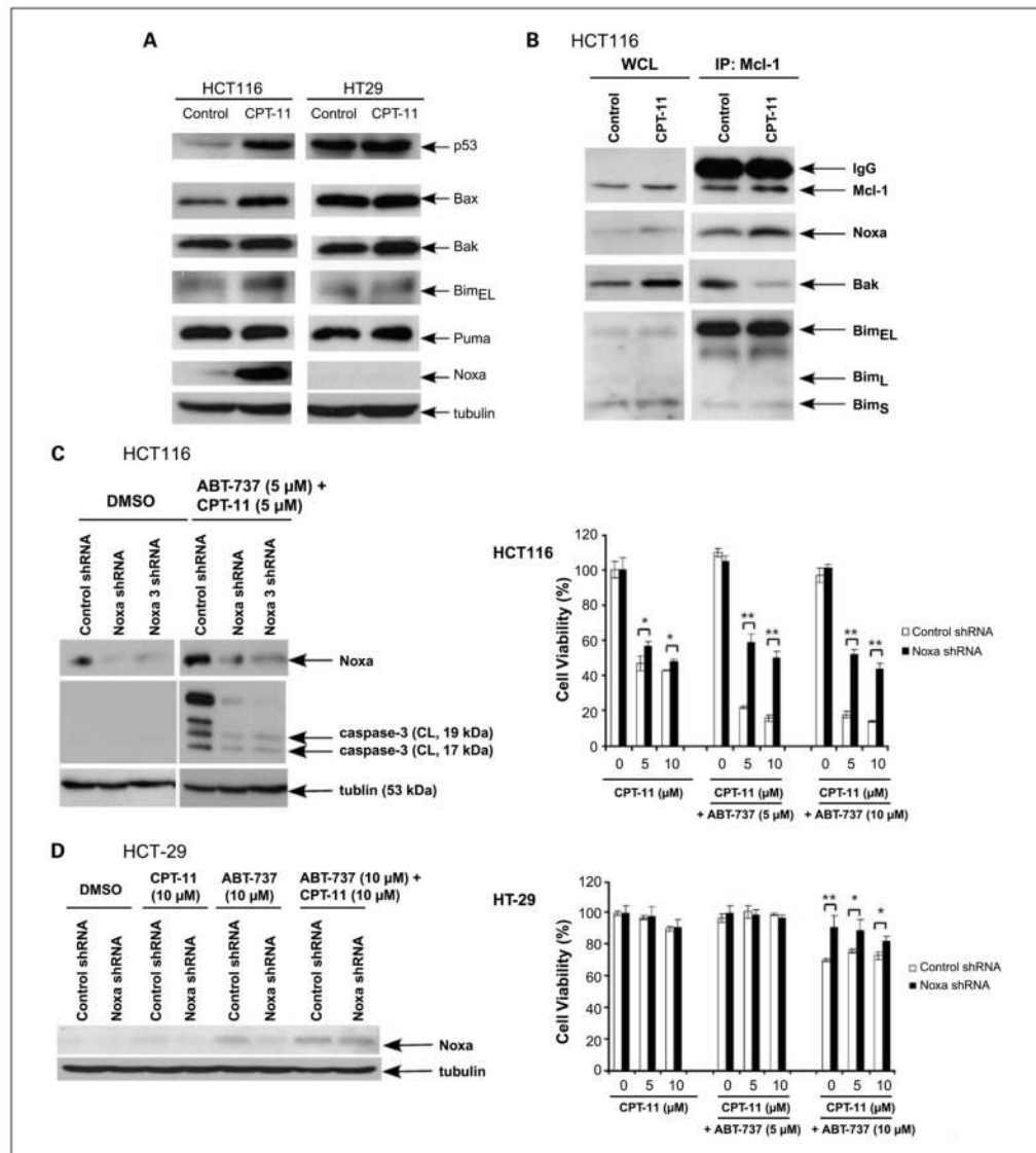
Fig. 6. CPT-11 up-regulates Noxa to sequester Mcl-1 and to disrupt Mcl-1/Bak complexes. Knockdown of Noxa attenuates the cytotoxicity of CPT-11 plus ABT-737. The effect of CPT-11 treatment on the expression of BH3-only and proapoptotic proteins was determined. A , HCT116 and HT-29 cells were incubated with CPT-11 (10 μmol/L) for 48 h and whole-cell lysates were subjected to immunoblot analysis for the expression of indicated proteins. B , HCT116 cells were treated with vehicle (DMSO) or CPT-11 (10 μmol/L) for 24 h and immunoprecipitation was done for Mcl-1 proteins. Whole-cell lysates from beads and eluted proteins from beads were separated by SDS-PAGE and then probed for Mcl-1, Bim, Noxa, or Bak proteins. C and D , knockdown of Noxa was achieved using lentiviral-delivered shRNA in HCT116 ( C , left) or HT-29 ( D , left) cells and the level of Noxa expression was determined in untreated (vehicle) and drug-treated cells by immunoblotting. HCT116 cells ( C , left) were treated with vehicle (DMSO) or the combination of ABT-737 and CPT-11 at the indicated doses for 24 h and caspase-3 cleavage was analyzed in whole-cell lysates subjected to immunoblotting. β-Tubulin served as a control for protein loading. We then determined the effect of Noxa knockdown versus control shRNA on cell viability in drug-treated HCT116
