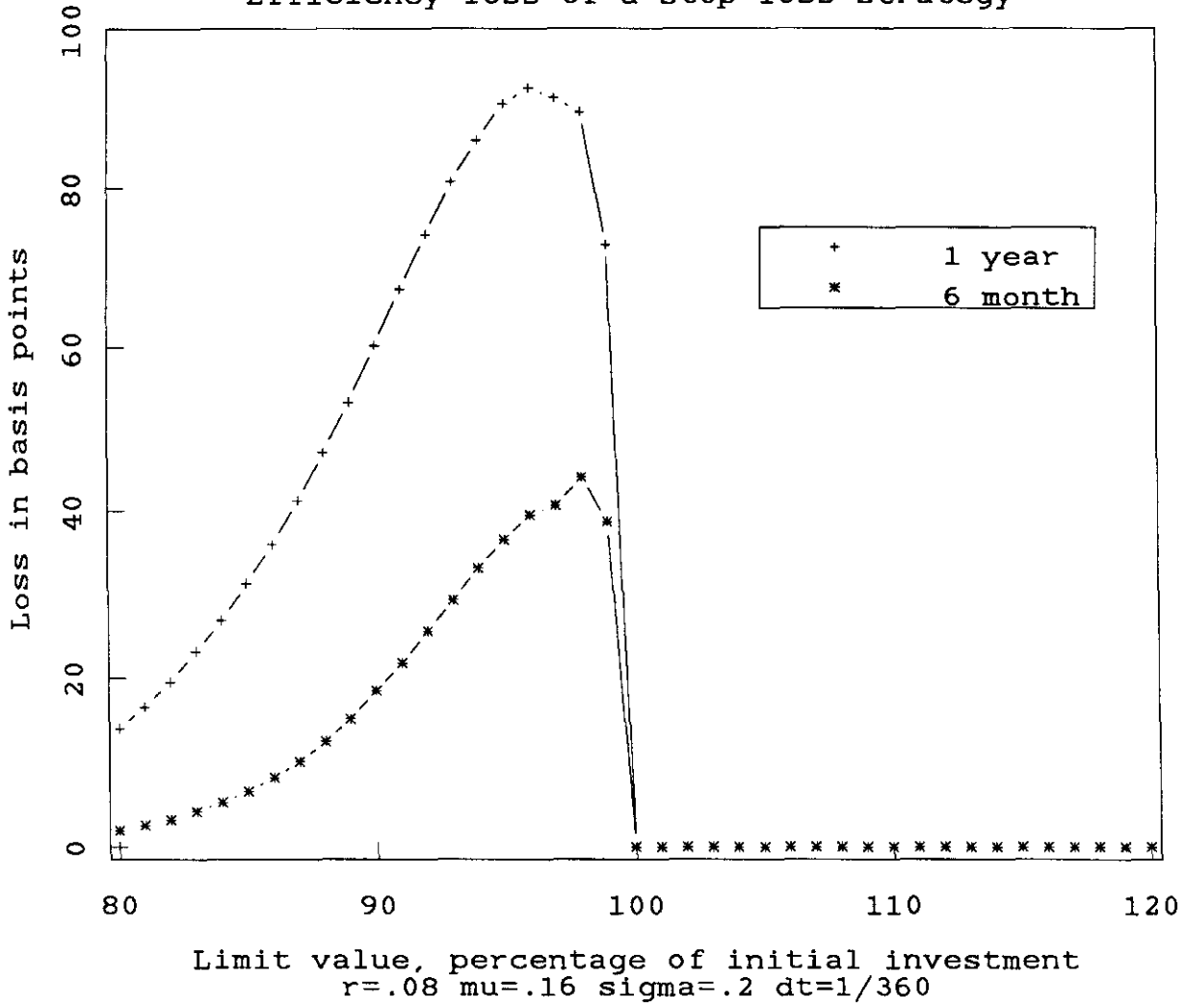
FIGURE 1 Efficiency loss of a stop-loss strategy
