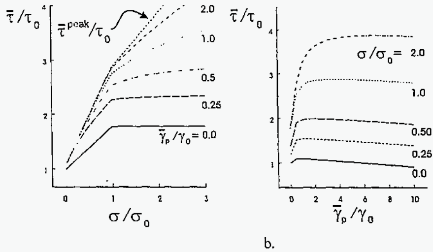
a. b. Figure 5: Results of modeling yield surfaces (a) and shear stress as a function of plastic shear strain \bar{\gamma}^p at constant mean stress (b). The curve marked \bar{\tau}^{peak}/\tau_0 in (a) shows peak stress as a function of \sigma . From numerical results the locus of peak stresses crosses the yield surfaces, indicating that peak stresses do not constitute a yield surface.
