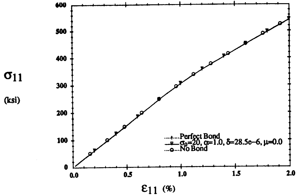
(a) Axial Response
