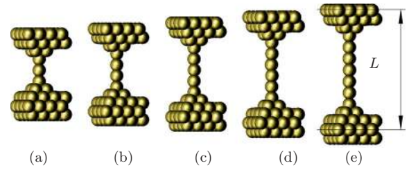
FIG. 8. (Color online) Generic gold wire supercells containing 3 to 7 atoms bridging pyramidal bases connected to stacked Au(100) layers. As indicated on the figure, the electrode separation L is defined as the distance between the plane in each electrode containing the second-outermost Au(100) layer.
