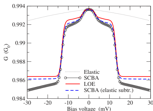
FIG. 11. (Color online) Elastic and inelastic differential conductance calculated at T=10.0 K in a reduced device region for the seven-atom wire shown in Fig. 10. The small variation in elastic conductance with bias (dotted curve) relates to a weak energy dependence of the elastic transmission function at the \Gamma point around \varepsilon_F . The full SCBA calculation (circles) follows this trend and shows on top of it symmetric drops characteristic for phonon scattering. The LOE calculation (line) does not include the elastic variation but gives basically the same predictions for the inelastic signals as the SCBA with the elastic background signal subtracted (dashed curve). This illustrates the agreement between the LOE and SCBA approaches for the inelastic contribution.
