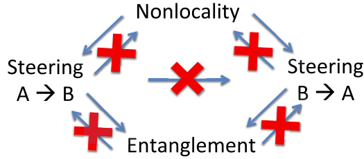
FIG. 1. (Color online) Relations between entanglement, one-way steering, two-way steering, and nonlocality. Nonlocality implies two-way steerability (i.e., from Alice to Bob and from Bob to Alice), while one-way steerability (i.e., from Alice to Bob or from Bob to Alice) implies entanglement. Here we show that the converse relations do not hold, considering arbitrary POVMs (red crosses).
