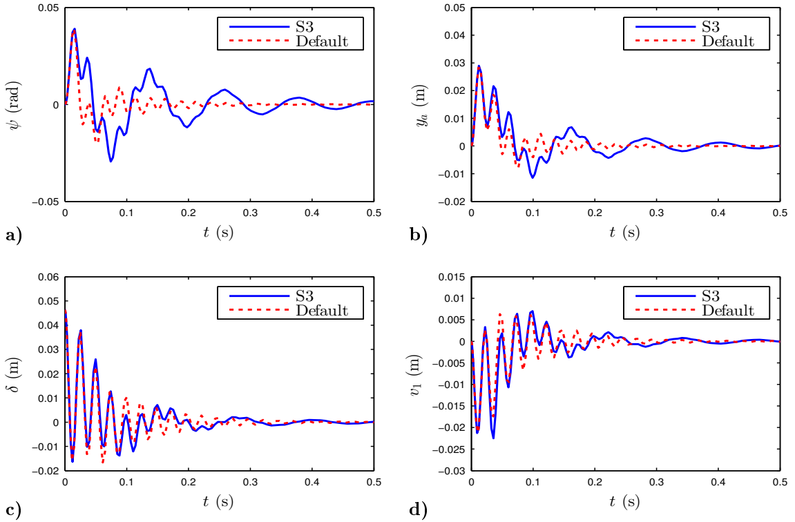
Fig. 6 Comparison of time-domain oscillations achieved by the default and S3 configurations ( \phi(t = 0) = 0.1 rad).
