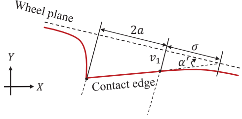
Fig. 3 Schematic of the straight tangent tire model.
