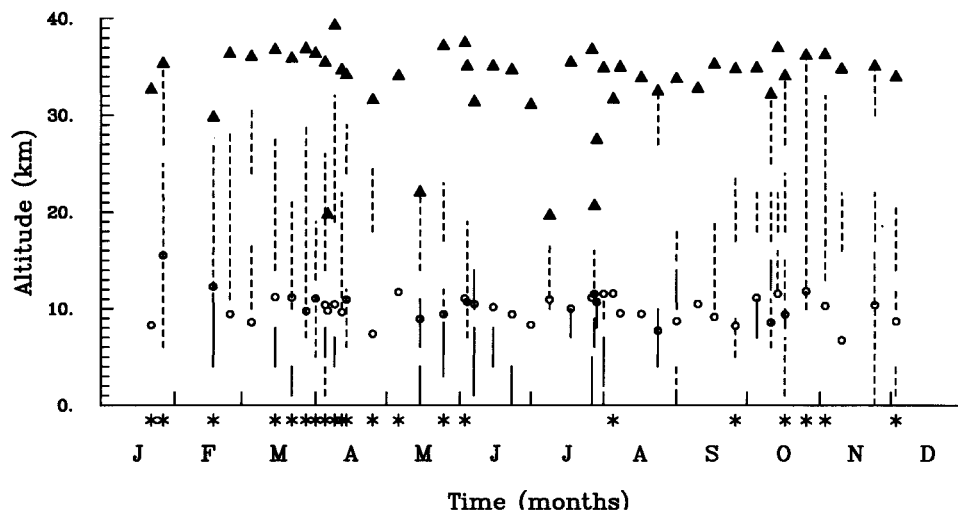
FIG. 1. Summary of the 47 ozonesonde flights. The maximum height reached is marked by the triangles and the circles show the tropopause height. Dashed lines mark those regions showing clear evidence of anticyclonic rotation in the hodographs. Similarly, the solid lines mark regions of cyclonic rotation. Asterisks mark the flights that passed the gravity wave test.
