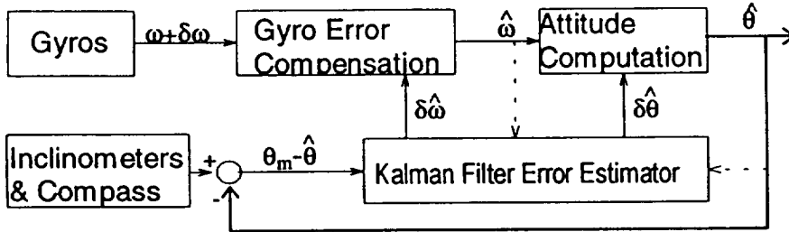
Figure 3: Complimentary Kalman filter for orientation
