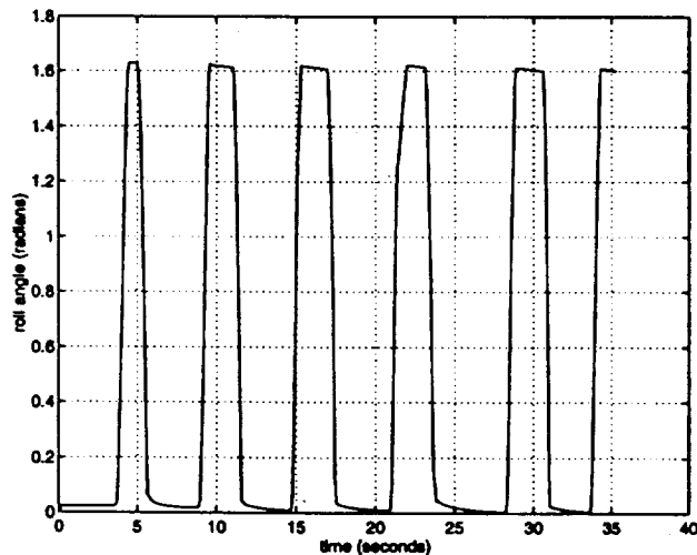
Figure 7: Test run with complimentary Kalman filter.
