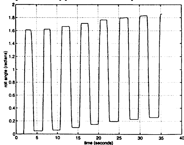
Figure 6: Test run without complimentary Kalman filter.
