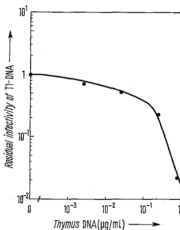
Fig. 2. Effect of heterologous DNA on the efficiency of infectious T1-DNA. Infectivity of native T1-DNA (0.2 µg/ml) is shown as a function of concentration of DNA prepared from calf thymus and added to a standard spheroplast assay
