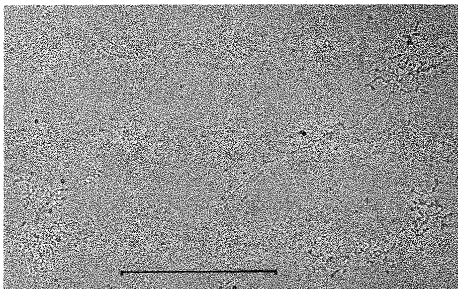
Fig. 8. a T1-DNA denatured by heat (non-infective), b "Heat-treated" T1-DNA (infective)
