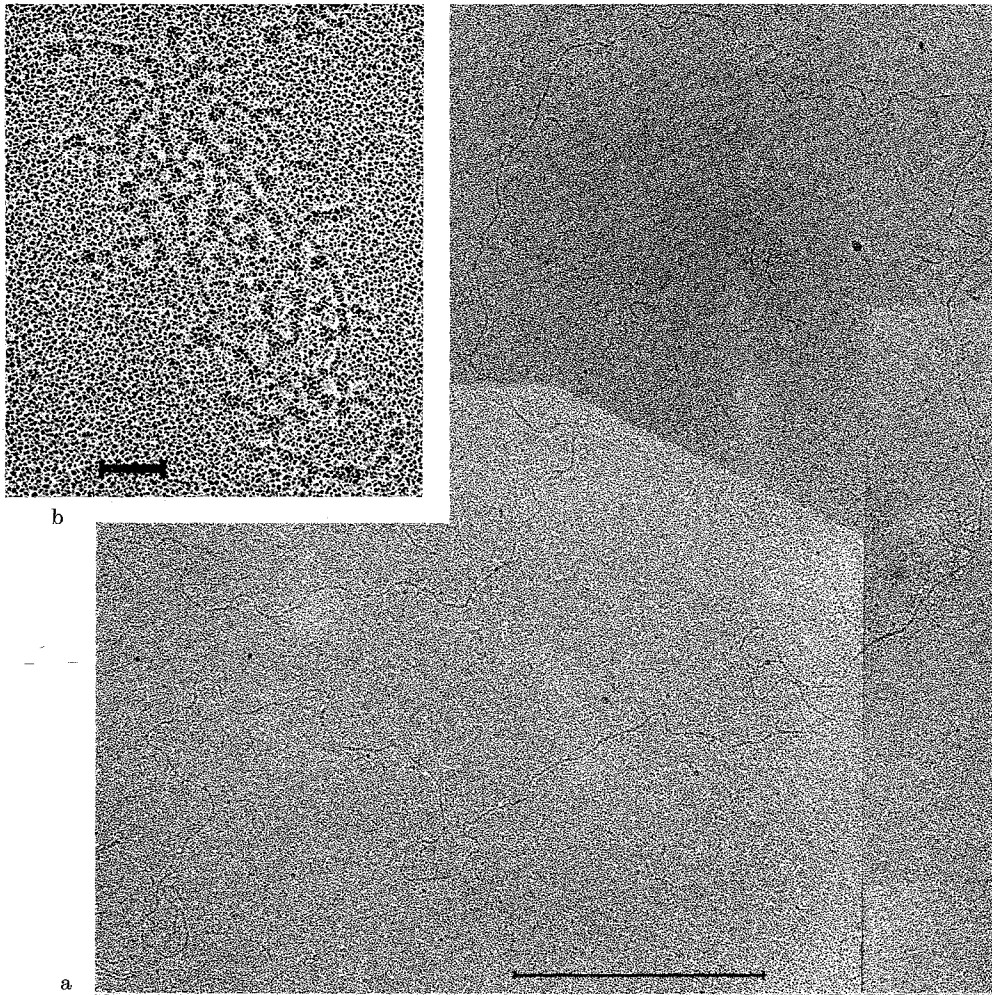
Fig. 7. a Native T1-DNA. This and the following samples were prepared according to the Kleinschmidt-technique at a DNA concentration of 2 \mu\text{g/ml} and photographed by Dr. H. FRANK (Max-Planck-Institut für Virusforschung, Tübingen). In this and all succeeding illustrations the scale mark represents 1 \mu , if not stated otherwise. b "Heat-treated" T1-DNA molecule, enlarged detail of Fig. 9. Scale mark represents 0.1 \mu .
