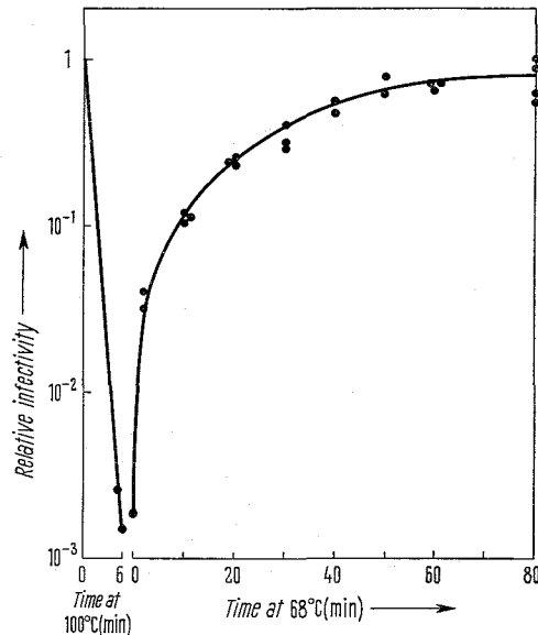
Fig. 5. Restoration of the infectivity of denatured T1-DNA. 10 \mu\text{g} DNA/ml M/100 NCE buffer were heated for 6 min in boiling water and thereafter quickly cooled in ice-water. The relative absorbance at 260 \text{ m}\mu was increased to 1.28 by this treatment. After dilution into M/5 NCE the DNA ( 5 \mu\text{g}/\text{ml} ) was immersed in a water-bath at 68^\circ\text{C} and portions were withdrawn at the time indicated. The assay on infectivity was performed at a DNA concentration of 0.025 \mu\text{g}/\text{ml} adsorption fluid
