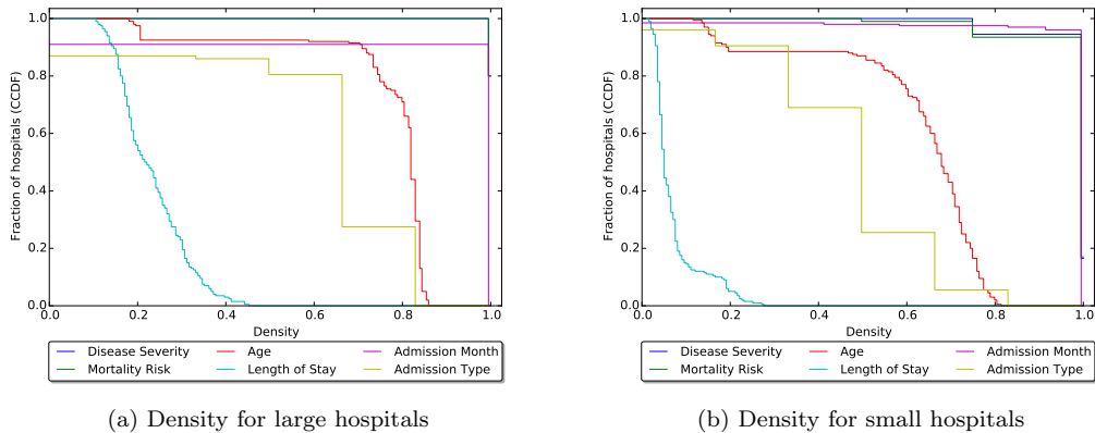
Figure 4: Density – Ratio of the number of values of an attribute present in a column to the total number of values of the attribute
