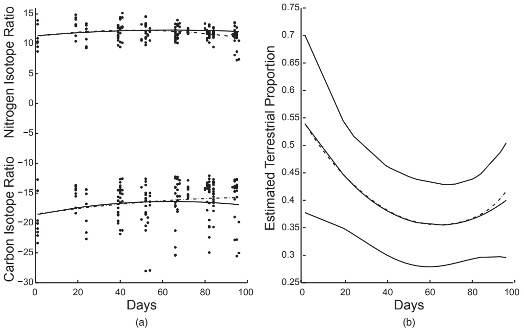
Fig. 3. (a) Observed and estimated (—) mean carbon and nitrogen IRs based on a quadratic fit to the logit of the population diet proportion associated with terrestrial source (·-·-·, estimate based on quadratic models for IRs) and (b) estimated population diet proportion associated with terrestrial source as a function of time, with pointwise 95% confidence interval, based on a quadratic logit model (·-·-·, indirect estimate based on quadratic models for IRs)
