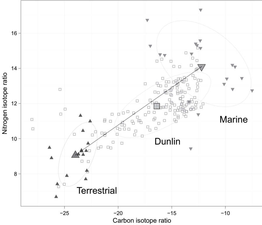
Fig. 1. Dunlin ( \square ) mixture and terrestrial ( \blacktriangle ) and marine ( \blacktriangledown ) discrimination-corrected source \delta^{13}\text{C} and \delta^{15}\text{N} observations with means and bivariate normal 75% data ellipses for reference: the line segment connects the discrimination-corrected source means
