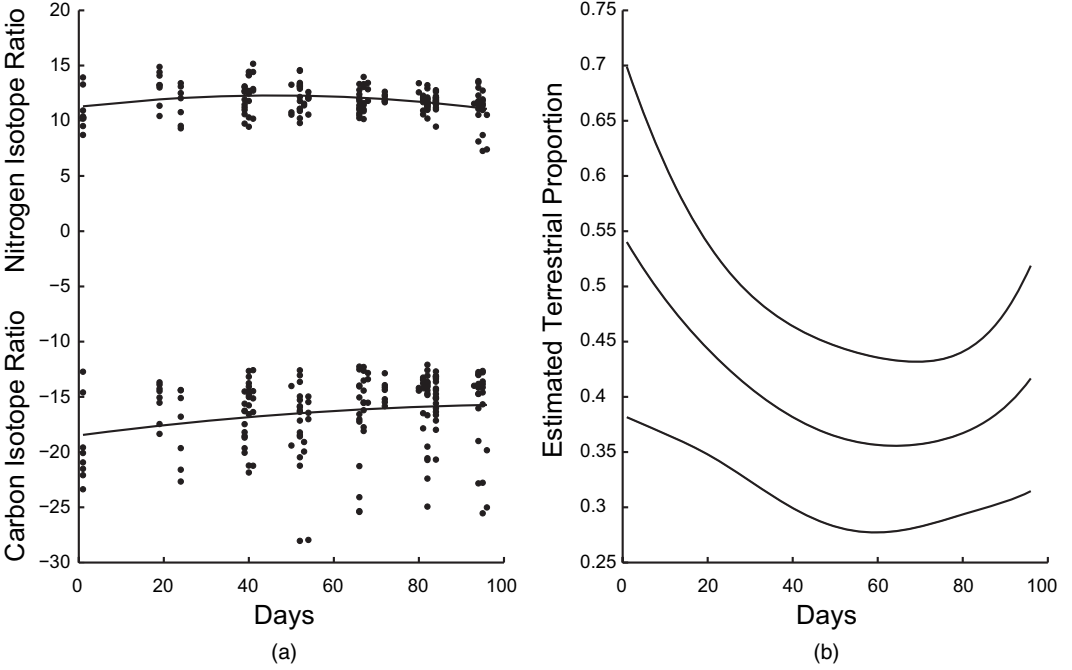
Fig. 2. (a) Observed carbon and nitrogen IRs with quadratic fits and (b) indirectly estimated population diet proportion associated with terrestrial source as a function of time, with pointwise 95% confidence intervals based on a quadratic fit
