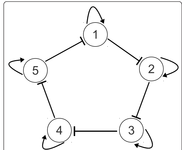
Figure 5 A standard repressilator structure. A repressilator structure with 5 nodes and auto-activation is shown in the figure. The mass-action type CRN model of this structure contains 51 distinct complexes and 55 reactions.
