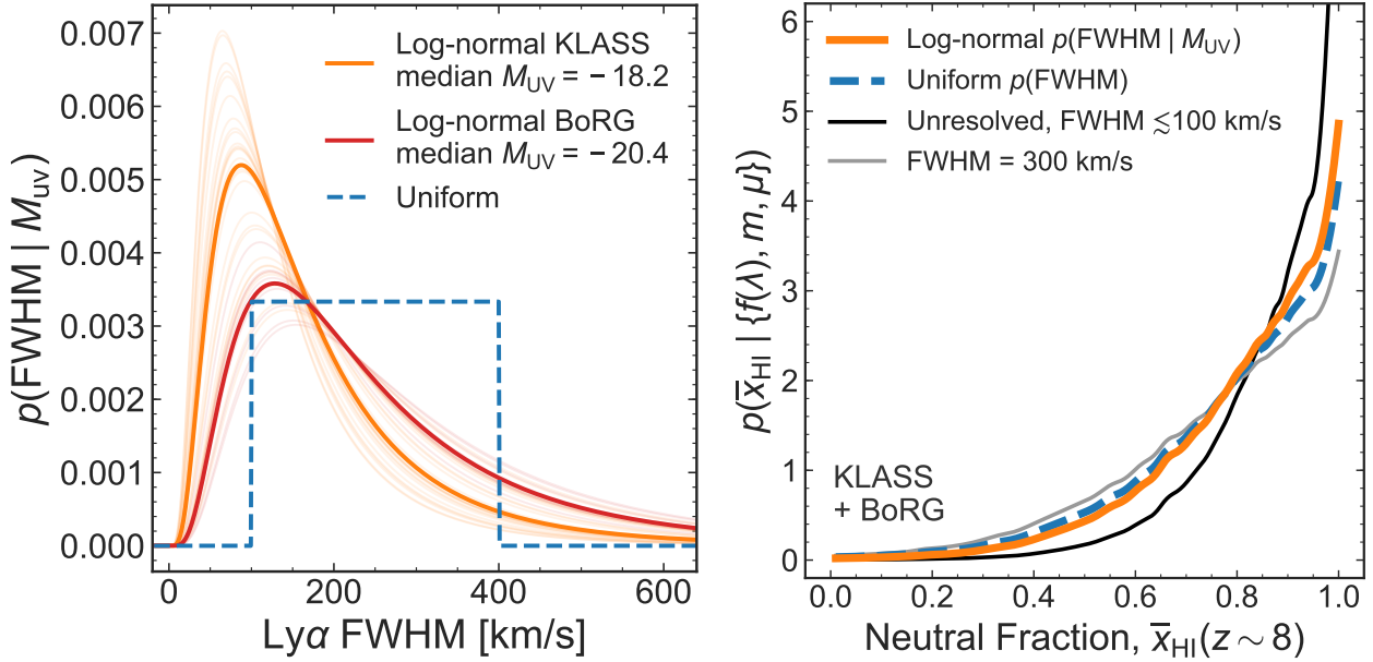
Figure C3. Left: Example prior probability distributions for Ly \alpha FWHM used in our inferences. The orange curves shows the log-normal priors p(\text{FWHM} | M_{\text{UV}}) for the KLASS sample (median M_{\text{UV}} = -18.2 shown as thick orange line), while the red curves shows the log-normal priors for the BoRG sample (prior for median M_{\text{UV}} = -20.4 is the thick red line). The blue dashed line shows a uniform prior (independent of M_{\text{UV}} ) between 100 – 400 km s ^{-1} . Right: Posterior probability distribution for the IGM neutral fraction derived from the KLASS and BORG samples using several different FWHM priors. The thin black line shows the posterior obtained assuming all lines are unresolved ( \text{FWHM} \lesssim 100 \text{ km s}^{-1} ) while the thin grey line is the posterior obtained assuming all emission lines are 300 km s ^{-1} , demonstrating how the posterior flattens with increasing linewidth as the EW sensitivity decreases. For our UV faint targets we expect the lines to be relatively narrow, so the 300 km s ^{-1} case is extreme. The orange solid line shows the posterior obtained using our log-normal FWHM prior p(\text{FWHM} | M_{\text{UV}}) calculated for each galaxy (described in Appendix C4), and the blue dashed line shows the posterior obtained using the uniform prior which is independent of M_{\text{UV}} . The difference in the 68% limits obtained using these two posteriors is negligible: \Delta \bar{x}_{\text{HI}} \sim 0.03 . Thus our results are robust for emission lines with widths \sim 100 - 400 \text{ km s}^{-1} .
