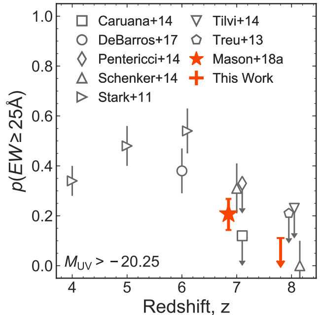
Figure 7. The redshift evolution of the ‘Ly \alpha fraction’ for UV faint galaxies, the fraction of LBGs observed with Ly \alpha EW \geq 25 Å. We plot literature measurements from Stark et al. (2011); Pentericci et al. (2014); Treu et al. (2013); Tilvi et al. (2014); Schenker et al. (2014); Caruana et al. (2014) and De Barros et al. (2017). We add small offsets in redshift for measurements at the same redshifts to ease the display of the data. We also plot the predicted Ly \alpha fraction from M18a calculating p(W > 25 | \bar{x}_{\text{HI}}, M_{\text{UV}}) using M_{\text{UV}} = -20 galaxies and the neutral fraction constraint \bar{x}_{\text{HI}} = 0.59^{+0.11}_{-0.15} (16 – 84% confidence intervals) as the orange star. We plot the upper limits recovered in this paper as orange lines, with the solid line showing our 68% confidence limit, and the dotted line extending to the 95% confidence limit. We calculate p(W > 25 | \bar{x}_{\text{HI}} > 0.76, M_{\text{UV}}) again using M_{\text{UV}} = -20 . Our constraint is consistent with literature values at the same redshift.
