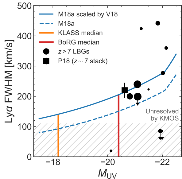
Figure C2. Ly \alpha spectral FWHM as a function of UV magnitude. Black circles are measurements from LBGs with confirmed z > 7 Ly \alpha (Oesch et al. 2015; Roberts-Borsani et al. 2016; Stark et al. 2017; Zitrin et al. 2015; Song et al. 2016a; Finkelstein et al. 2013; Shibuya et al. 2012; Ono et al. 2012; Schenker et al. 2012; Vanzella et al. 2011; Laporte et al. 2017a). The black square shows median values derived from a z \sim 7 sample by Pentericci et al. (2018). The blue dashed line shows the M18a, model for velocity offset ( \Delta v ) as a function of UV magnitude and redshift (via halo mass). The blue solid line shows the M18a model scaled by the FWHM -\Delta v_{\text{Ly}\alpha} relation presented by Verhamme et al. (2018). The grey hatched region shows FWHM unresolved by KMOS ( \lesssim 4 \text{ \AA} or \lesssim 110 \text{ km s}^{-1} ). The orange (red) vertical line shows the median UV magnitude of the KLASS (BoRG) samples.
