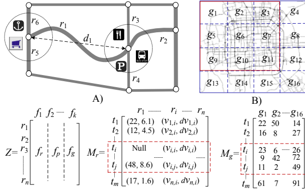
Figure 3. Context Extraction
