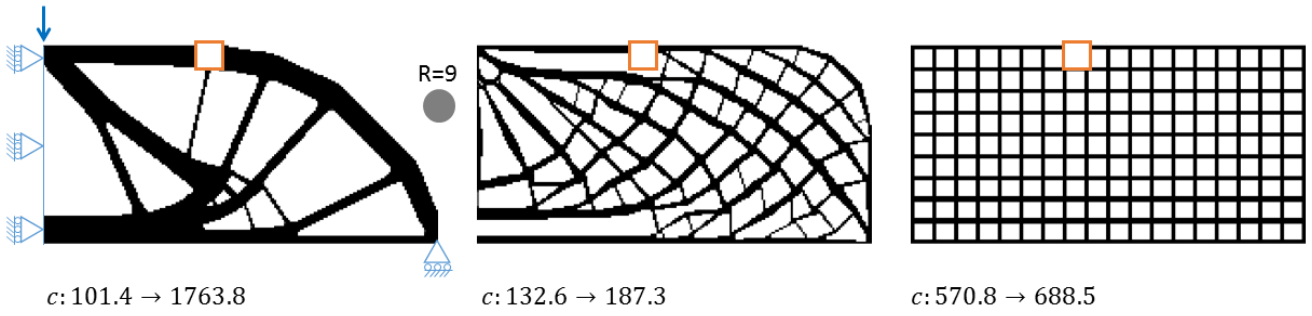
Fig. 12: Illustration of local material damage. Without damage, the structure constrained to a total volume (left) has the smallest compliance c of the three structures. When damaged as indicated by the orange square, this structure’s compliance becomes worst. The middle structure was generated by constraining the local volume limit. A regular grid structure (right) serves as reference.
