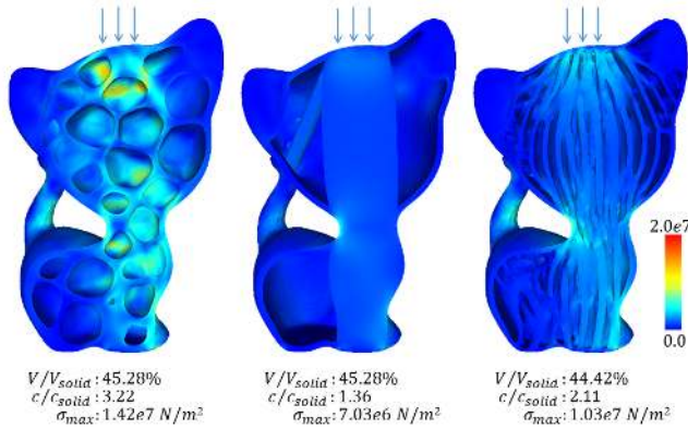
Fig. 17: Comparison between the honeycomb structure [12] (left, model courtesy of Lu et al. ) and structures generated by topology optimization with a total volume constraint [29] (middle) and with local volume constraints (right).
