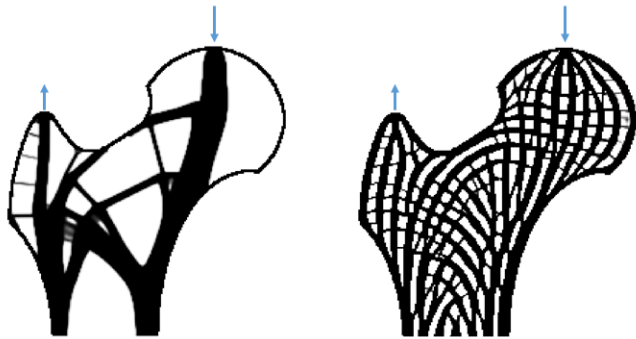
Fig. 10: Topology optimization in a 2D femur-shaped design domain. Left: Classical topology optimization with a total volume constraint. Right: Proposed topology optimization with local volume constraints.
