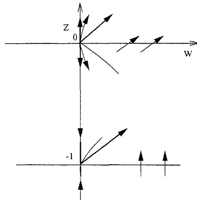
FIGURE 3. Phase plane related to (4.2), with q = \frac{\beta}{1+\gamma} .
