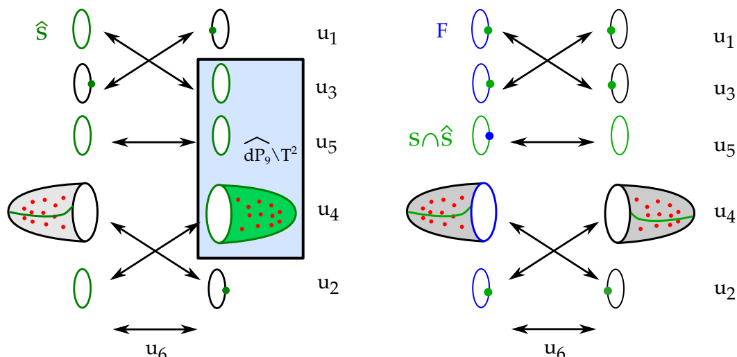
Figure 4. The Schoen Calabi-Yau threefold as a connected sum. The figure on the left shows the surface \widehat{S} in green. The figure on the right shows the divisor F = \mathbb{E} \times \widehat{\mathbb{E}} in blue and the intersection S \cap \widehat{S} in green. The coordinates are labeled by u_1, \dots, u_6 .
