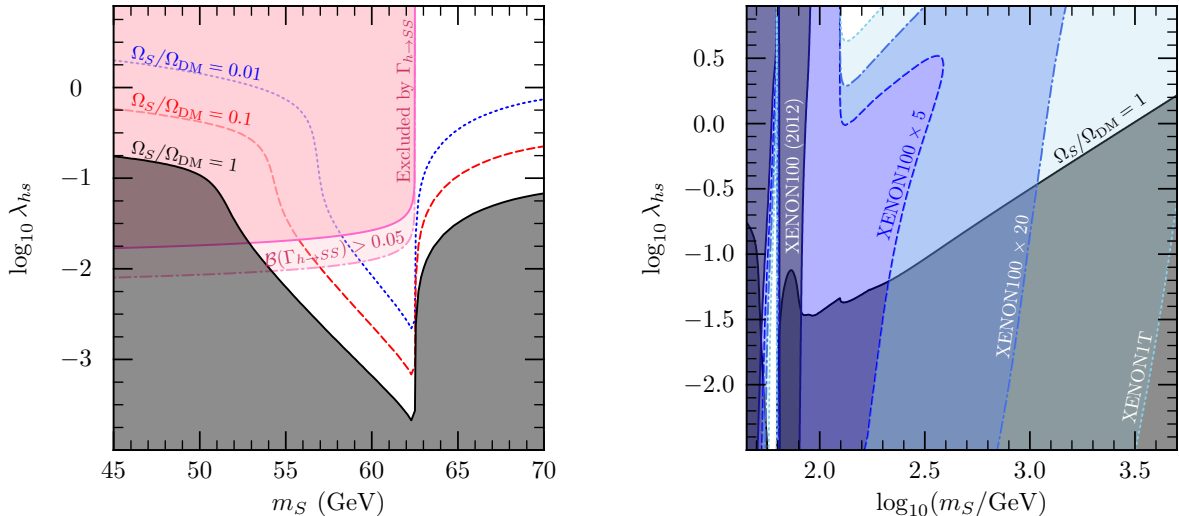
Figure 1: DM exclusion contours from Ref. [52] on the \lambda_{hs} , m_s plane. Left plot is a close-up on the region m_s \lesssim m_h/2 . The dark-shaded lower region is ruled out by the upper bound on the singlet DM relic density, \Omega_S/\Omega_{\text{DM}} \leq 1 . The region in the upper-left corner is ruled out by constraints on invisible Higgs decays. Right plot is over a wide mass range 45 \text{ GeV} \leq m_s \leq 5 \text{ TeV} . The DM relic density exclusion is shown superimposed with the current bound from XENON100 and bounds from future direct detection experiments (in lighter shades of blue).
