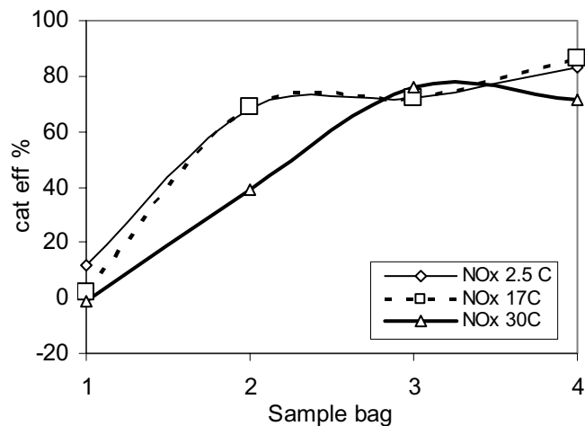
Figure 22 NOx conversion efficiency of TWC at different ambient temperature for LU-TJTC test
