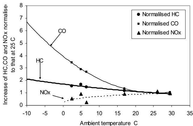
Figure 38 Relative increases of HC, CO and NOx for the first phase of the LU-TJTC test, normalized to the values at 25 °C
