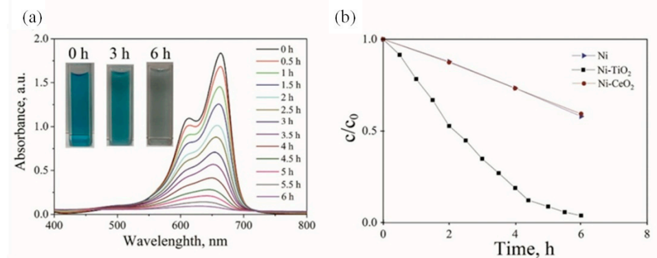
Figure 14. UV-Vis spectra of Ni-TiO 2 in MB aqueous solution (a); Photocatalytic degradation of MB at Ni, Ni-CeO 2 , Ni-TiO 2 (b).
