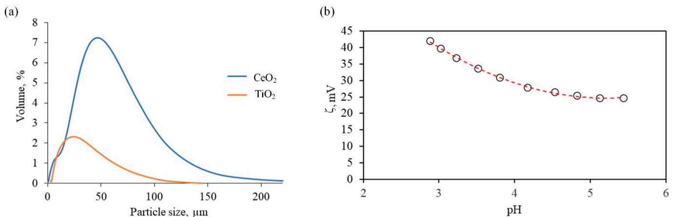
Figure 1. Particle size distribution for CeO 2 and TiO 2 (a) and \zeta -potential versus pH for CeO 2 (b).
