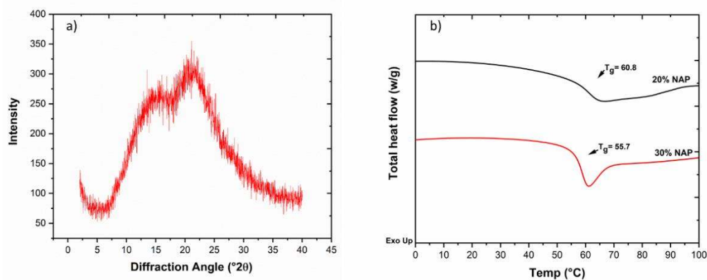
Figure 6. (a) Diffractogram from the 3D-printed tablets containing 30% NAP; (b) DSC thermogram of tablets containing 20% and 30% NAP.
