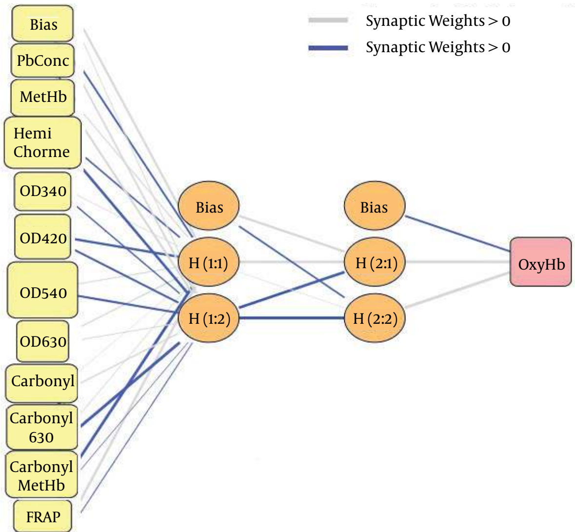
Figure 4. Feed-Forward Architecture for the Artificial Neural Network as a Multilayer Perceptron (11,2,2,1).
