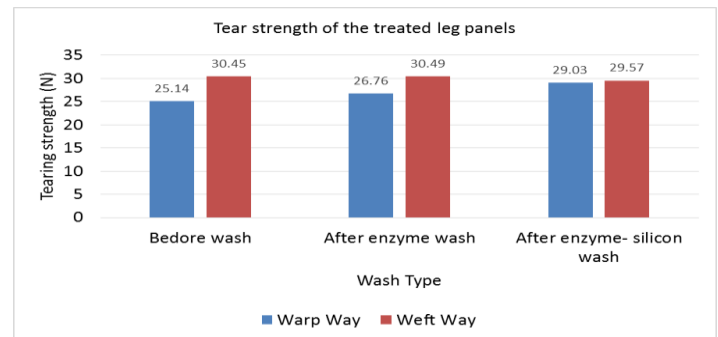
Fig. 2. Changes in fabric tearing strength in before wash, after enzyme wash and after enzyme- silicone wash
