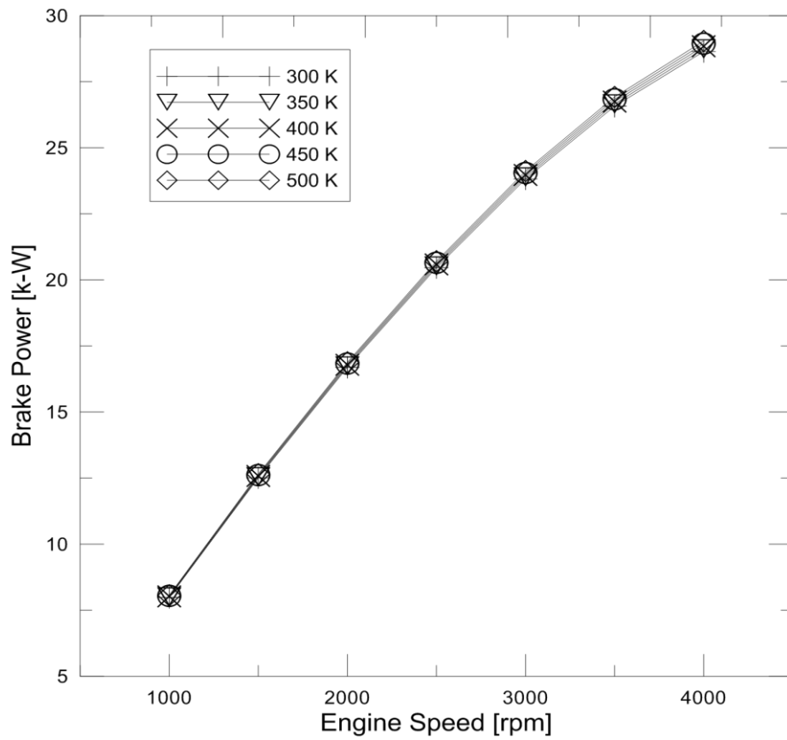
Figure 3. Variation of brake power with engine speed.
