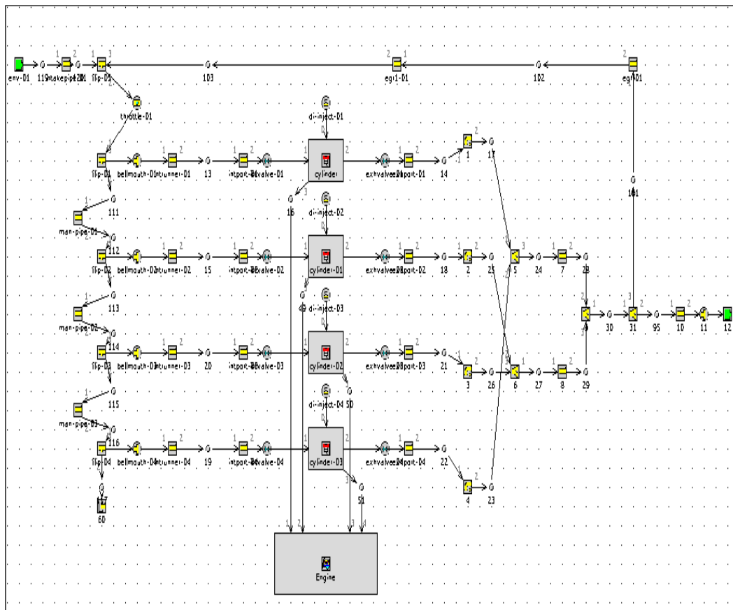
Figure 1. Computational model of the engine.
