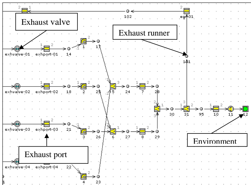
Figure 2. Exhaust system components.
