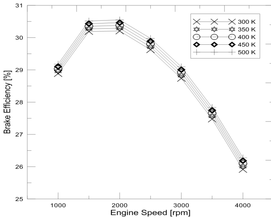
Figure 4. Effect of engine speed variation on brake thermal efficiency.
