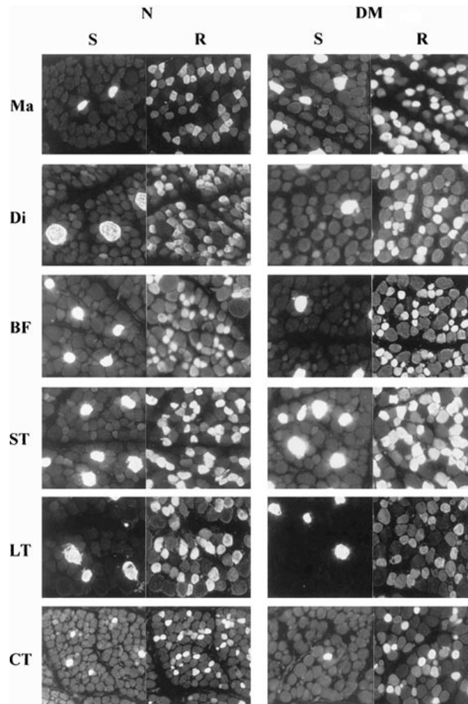
Figure 2. Immunohistochemical analysis of transverse serial sections of the muscles Masseter (Ma), Diaphragma (Di), Biceps femoris (BF), Semitendinosus (ST), Longissimus thoracis (LT) and Cutaneous trunci (CT) excised from normal (N) and double-muscled (DM) 180-day-old foetuses and reacted with monoclonal antibodies raised against slow (S) and fast (R) MHC. The labelling with antibodies raised against embryonic MHC (E), foetal MHC (F) and alpha-cardiac MHC (A) was not shown. The first generation was composed of fibres only recognised by S observed in all muscles of both genotypes and fibres labelled with S, E, F, A only present in Ma. The second generation of fibres was composed of fibres only recognised by S, R, E, F, A corresponding to type IIC fibres; cells recognised by R, E, F, A; fibres recognised by E, F, A and fibres only labelled with R.
