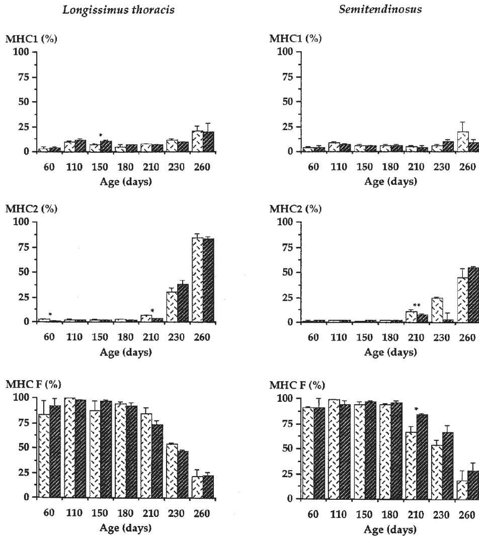
Figure 5. Evolution of MHC1, MHC2 and foetal MHC percentages in Longissimus thoracis and Semitendinosus muscles of normal and double-muscular foetuses at different stages of development.
