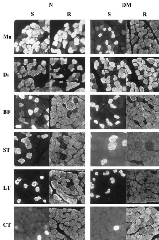
Figure 3. Immunohistochemical analysis of transverse serial sections of the muscles Masseter (Ma), Diaphragma (Di), Biceps femoris (BF), Semitendinosus (ST), Longissimus thoracis (LT) and Cutaneous trunci (CT) excised from normal (N) and double-muscled (DM) 260-day-old foetuses and reacted with monoclonal antibodies raised against slow MHC (S) and fast (R) MHC. The labelling with antibodies raised against embryonic MHC (E), foetal MHC (F) and alpha-cardiac MHC (A) was not shown. Fibres of the first generation were only recognised by S corresponding to adult type I fibres. The second generation of fibres was composed of fibres only recognised by S, R, E, F, A corresponding to type IIC fibres; fibres recognised by R, E, F, A; fibres recognised by E, F, A; fibres only labelled with R corresponding to adult type IIA and IIB fibres; fibres recognised by S, E, F, A only observed in Di and Ma.
