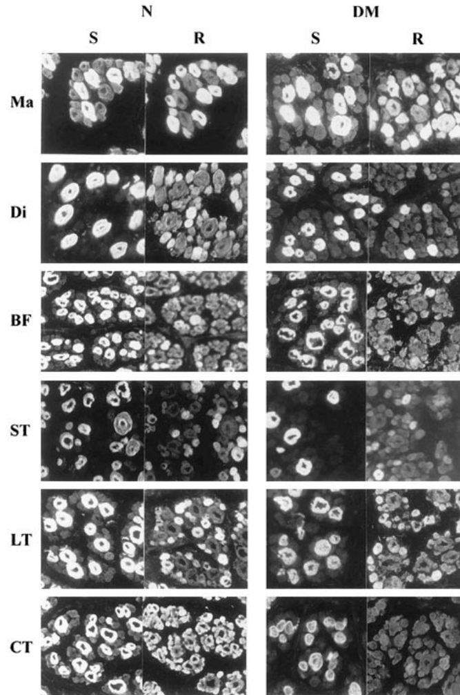
Figure 1. Immunohistochemical analysis of transverse serial sections of the muscles Masseter (Ma), Diaphragma (Di), Biceps femoris (BF), Semitendinosus (ST), Longissimus thoracis (LT) and Cutaneus trunci (CT) excised from normal (N) and double-muscled (DM) 110-day-old foetuses and reacted with monoclonal antibodies raised against slow (S) and fast (R) MHC. The labelling with antibodies raised against embryonic MHC (E), foetal MHC (F) and alpha-cardiac MHC (A) was not shown. Large myotubes were recognised by S, R, E, F, A and others were recognised by S, E, F, A. They corresponded to the first generation of fibres. The second generation of fibres was composed of smaller myotubes recognised by S, R, E, F, A or by R, E, F, A and very small fibres recognised by E, F, A.
