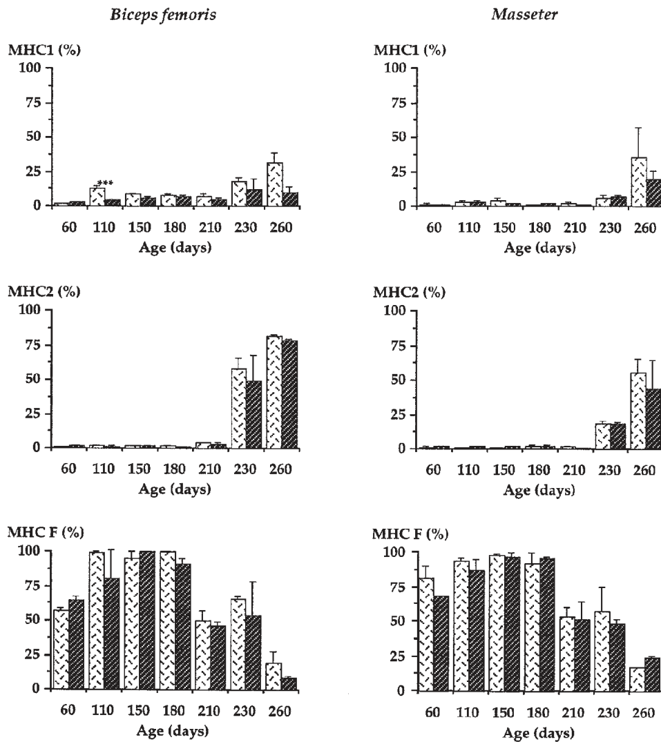
Figure 6. Evolution of MHC1, MHC2 and foetal MHC percentages in Biceps femoris and Masseter muscles of normal (hatched) and double-muscled (solid black) foetuses at different stages of development.
