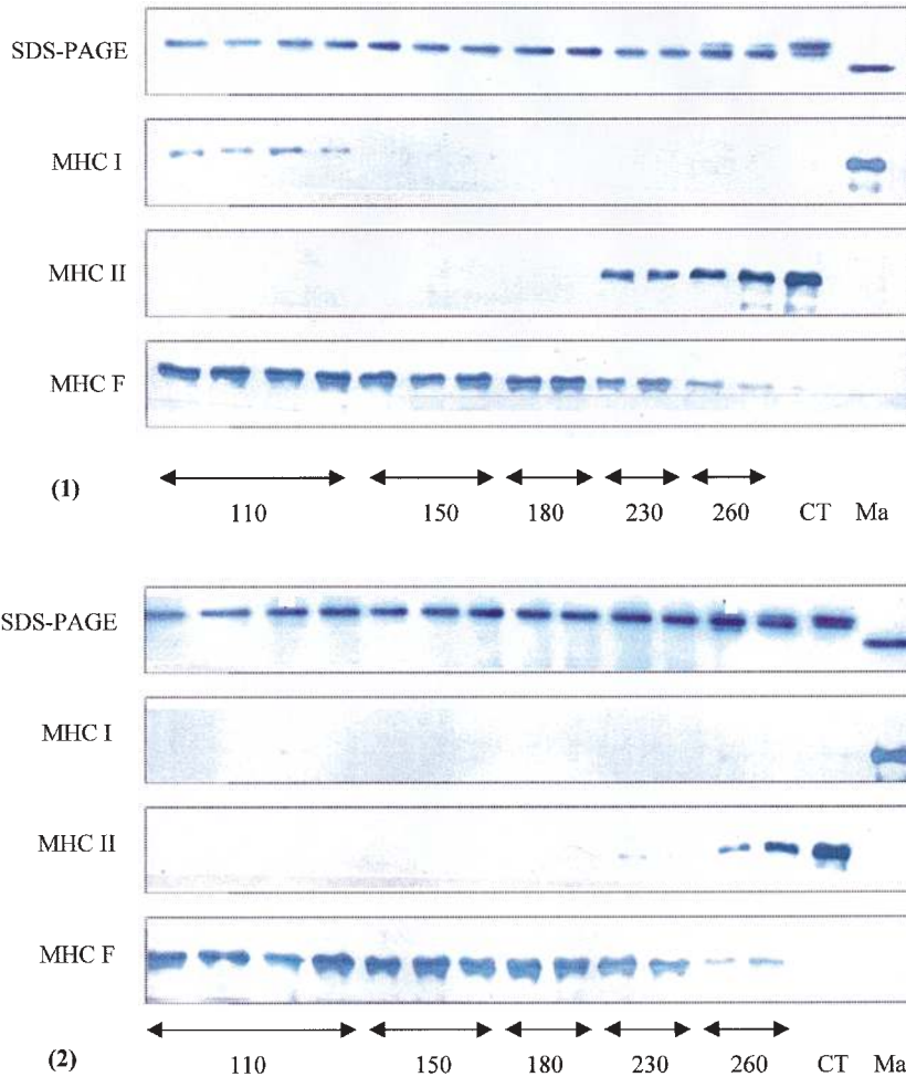
Figure 7. Different myosin heavy chains revealed by immunoblotting in N and DM Cutaneus trunci (CT) muscle from 110 to 260 days of foetal life. (1) Normal; (2) Double-muscled. CT: adult CT muscle; Ma: adult Masseter muscle. MHC I: slow MHC; MHC II: fast MHC 2a and 2b; MHC F: foetal MHC.
