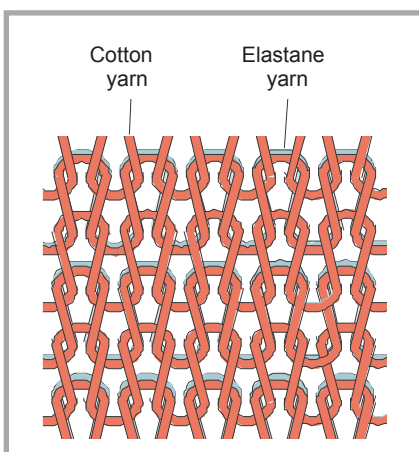
Figure 1. Knitted fabric with platted elastane yarn in every second course.
