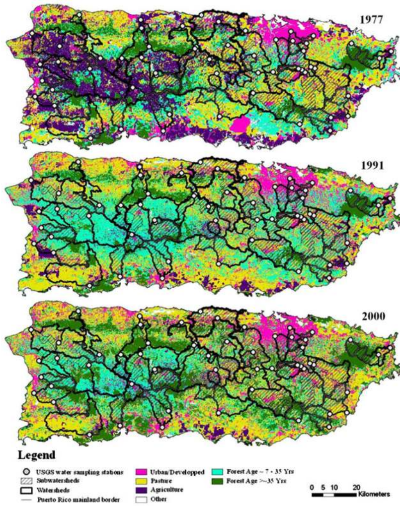
Fig. 1. Distribution of LUC classes used in the analyses shown over the study watersheds
