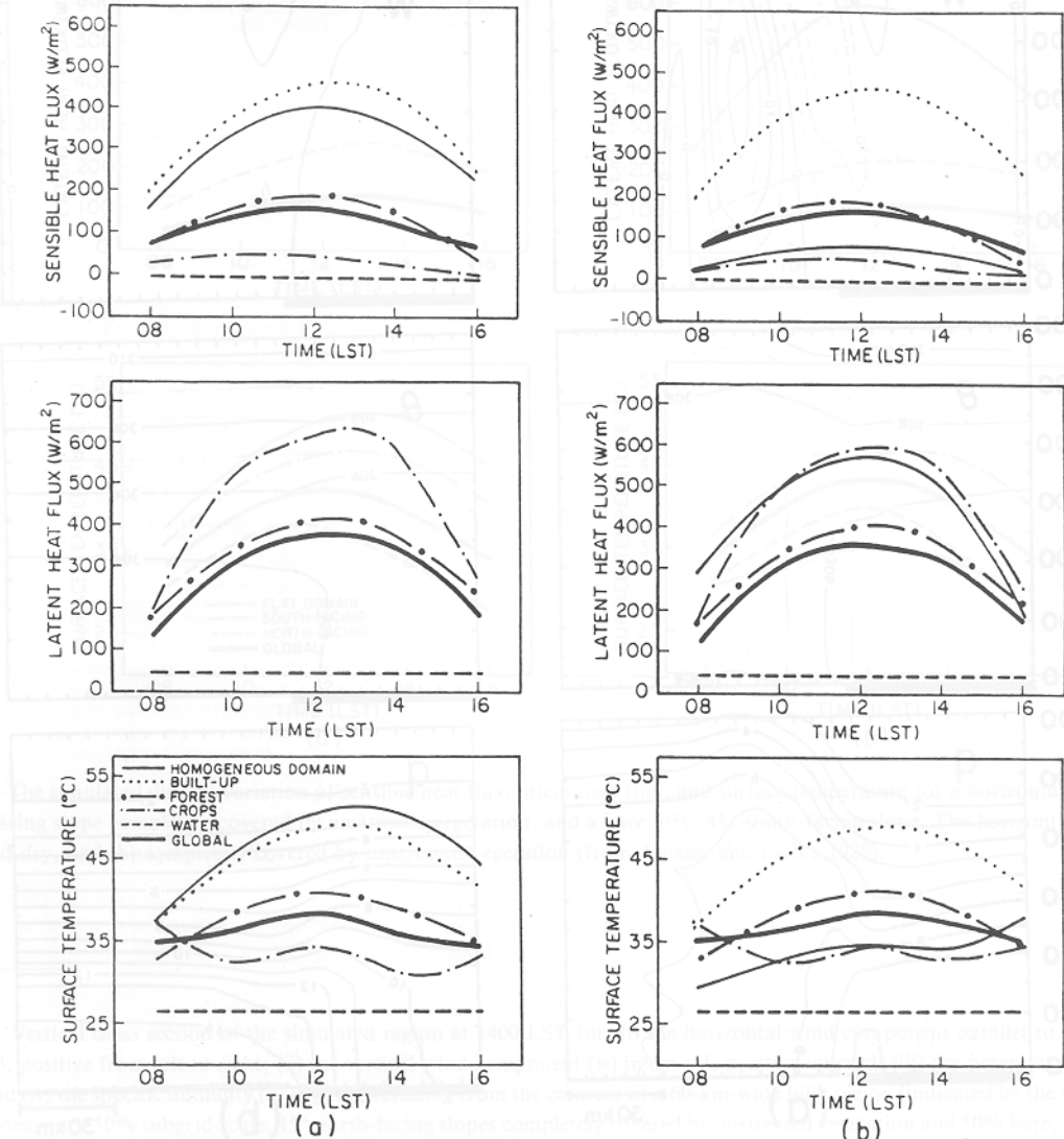
Fig. 21. The diurnal variation of sensible heat flux, latent heat flux, and surface temperature simulated for a heterogeneous land surface which consists of 20% built-up areas and waste lands, 10% bodies of water, 40% agricultural crops, and 30% forests. The global values represent the weighted average of the values for the heterogeneous region. The heterogeneous region is juxtaposed with (a) bare, dry land, and (b) land completely covered by unstressed vegetation (from Avissar and Pielke 1989).
