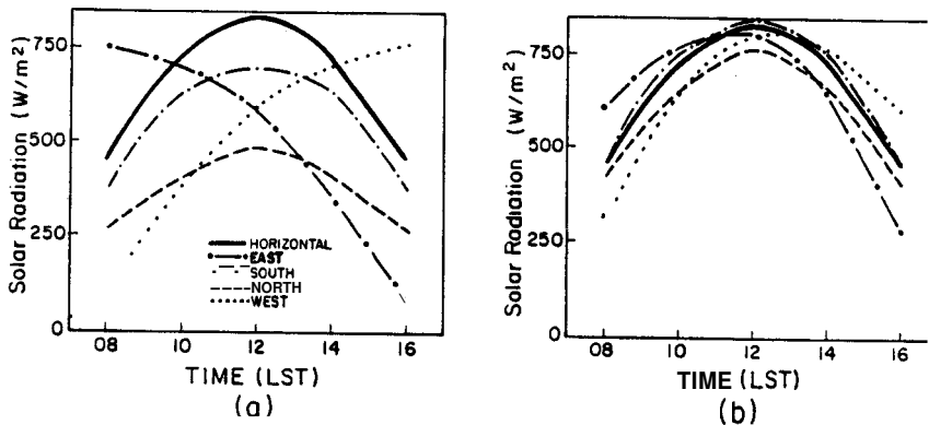
Fig. 17. The diurnal variation of solar global radiation received at the surface of a horizontal surface and on slopes facing north, east, west, and south, on July 15 at a latitude of 37°N. The slopes inclinations are (a) 45°, and (b) 15° (from Avissar and Pielke 1989).
