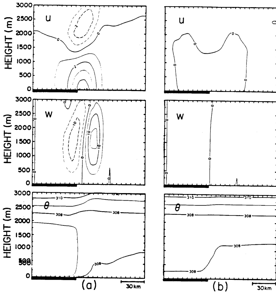
Fig. 16. Vertical cross section of the simulated region at 1400 LST for: (i) the horizontal wind component parallel to the domain ( u ) in m s^{-1} , positive from left to right; (ii) the vertical wind component ( w ) in cm s^{-1} , positive upward; and (iii) the potential temperature ( \theta ) in K, resulting from the contrast of a 60-km-wide hilly region (indicated by the dark underbar) which consists of 50% north-facing and 50% south-facing subgrid-scale dry slopes, and a 90-km wide dry flat region. The inclinations of the slopes are (a) 45°, and (b) 15° (from Avissar and Pielke 1989).
