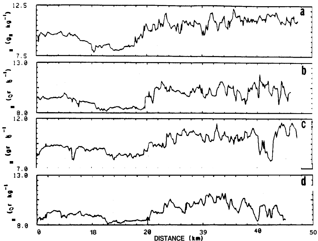
Fig. 6. The same as in Fig. 5 except for moisture mixing ratio (from Segal et al. 1989).
