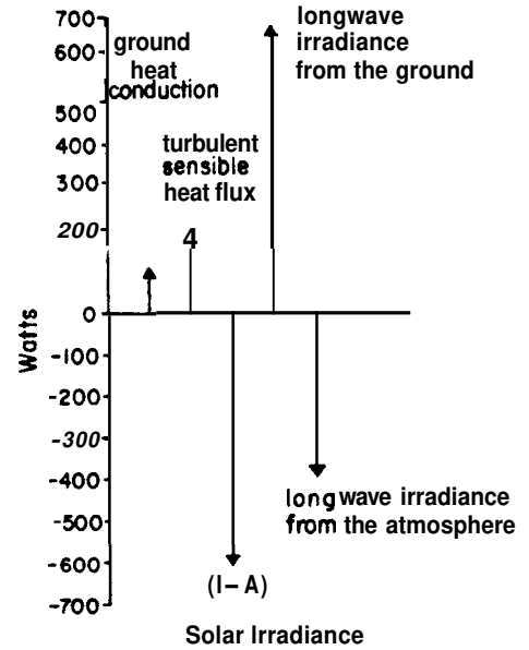
Fig. 3. Average heat fluxes at 1300LST observed over the Empty Quarter of Saudi Arabia. A positive value represents a loss to the surface and a negative value is a gain. The sum of the fluxes equals zero. Over the Empty Quarter, the latent heat flux is essentially zero (from Eric Smith, CSU, 1982, personal communication and Pielke, 1984).
