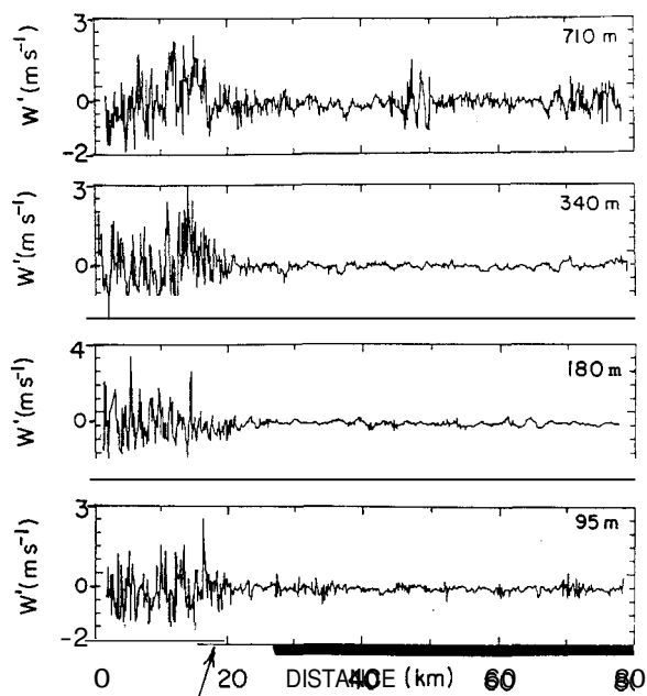
Fig. 12. Same as Fig. 10 except for vertical velocity (from Cramer 1988).
