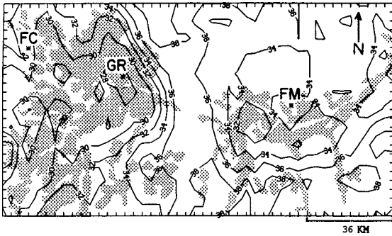
Fig. 4. Composite of GOES derived surface temperature at 1300 LST for the period 1 August 1986 to 15 August 1986 for northeast Colorado (FC-Fort Collins; FM-Fort Morgan; GR-Greeley; W-Windsor; B-Briggsdale). Irrigated areas are shaded (from Segal et al. 1988).
