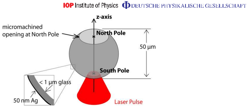
Figure 1. A glass hollow microsphere, with an \sim 50 nm silver coating on its \leq 1\ \mu\text{m} thick wall, is struck by a laser pulse at the ‘south pole’. TNSA protons are emitted through a circular opening at the ‘north pole’ and post-accelerated.
