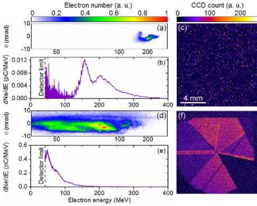
FIG. 1. Single shot raw Lanex images, energy spectra, and X-ray beam images obtained after a 10 mm long, 178 \mu\text{m} diameter capillary tube for two values of the plasma electron density (a) to (c): n_e = (5.4 \pm 0.3) \times 10^{18} \text{ cm}^{-3} ; (d) to (f): n_e = (8.1 \pm 0.5) \times 10^{18} \text{ cm}^{-3} .
