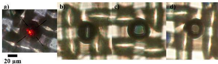
Figure 6.10. Laser micromachining: a) Premachined sphere showing the red confocal alignment laser reflection. Openings of different shapes are possible, b) slit, c) square and d) round, demonstrating the resolution and accuracy of the home-built laser micromachining set-up
