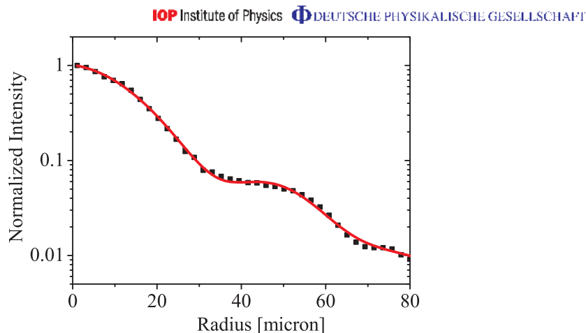
Figure 6. Normalized laser intensity distribution averaged over the azimuthal angle measured in the experiment (squares) and its multi-picks approximation used in simulations (the solid line).
