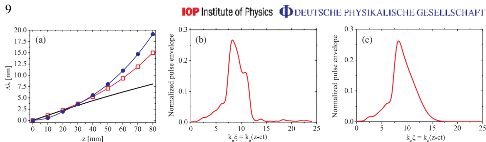
Figure 4. (a) The same as in figure 3(a) for a capillary filled with 40 mbar of hydrogen and laser pulse intensity I_0 = 1.3 \times 10^{17} \text{ W cm}^{-2} and an energy of 0.12 J. (b) Normalized laser pulse envelope a(r=0, \xi) on the axis at a distance of 70 mm with OFI included. All parameters are the same as in (a). (c) The same as in (b), but in pre-ionized plasma.
