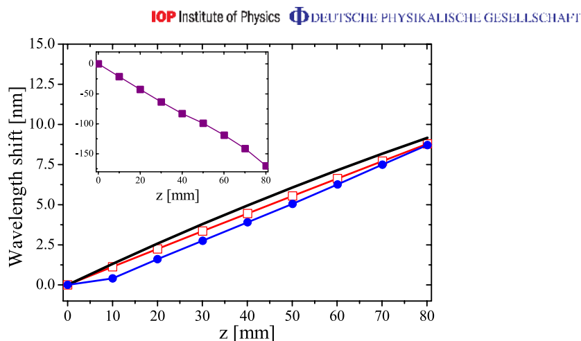
Figure 1. Wavelength shift calculated with (12), the solid line (not marked), and obtained in simulations as functions of the laser propagation distance in a capillary filled with 20 mbar of hydrogen; lines with markers: OFI included (dots) and pre-ionized plasma (open squares). The inset shows the wavelength shift for the same parameters but in a capillary filled with helium. Parameters are indicated in the text.
