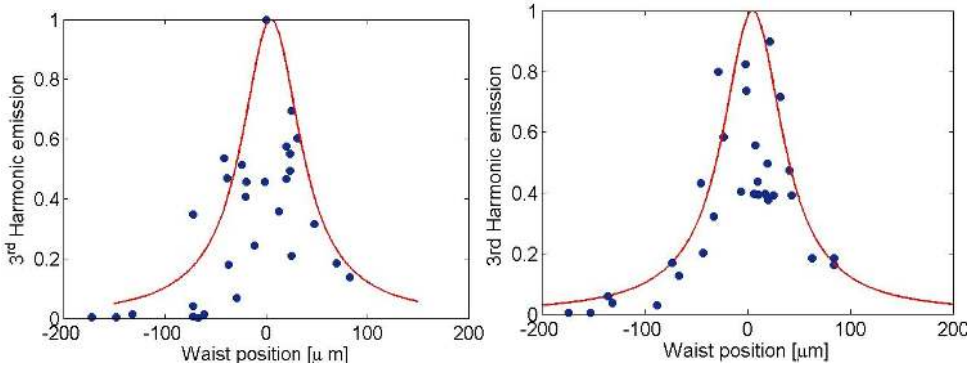
Figure 4: Total harmonic yield for 3 rd harmonic for low contrast( 10^{-7} ) (left) and high contrast ( 10^{-8} ) (right) of the incident laser pulse. Red lines indicate the Gaussian fit for the incident laser pulse intensity.
