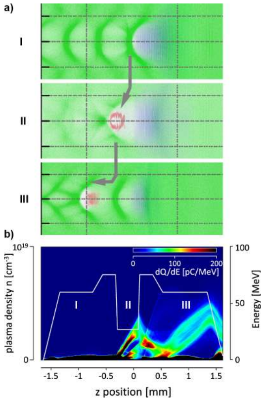
FIG. 6: a) Plasma electron density distribution (green), accelerated electron bunch (red) and laser pulse (blue) shown at the axial section for the instant of laser pulse passing the corresponding density regions I-III. b) same as in Fig. 5.
