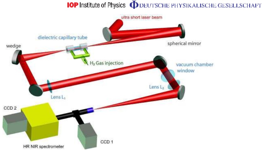
Figure 5. Schematic view of the experimental setup. All the elements up to the vacuum chamber window were under vacuum.
