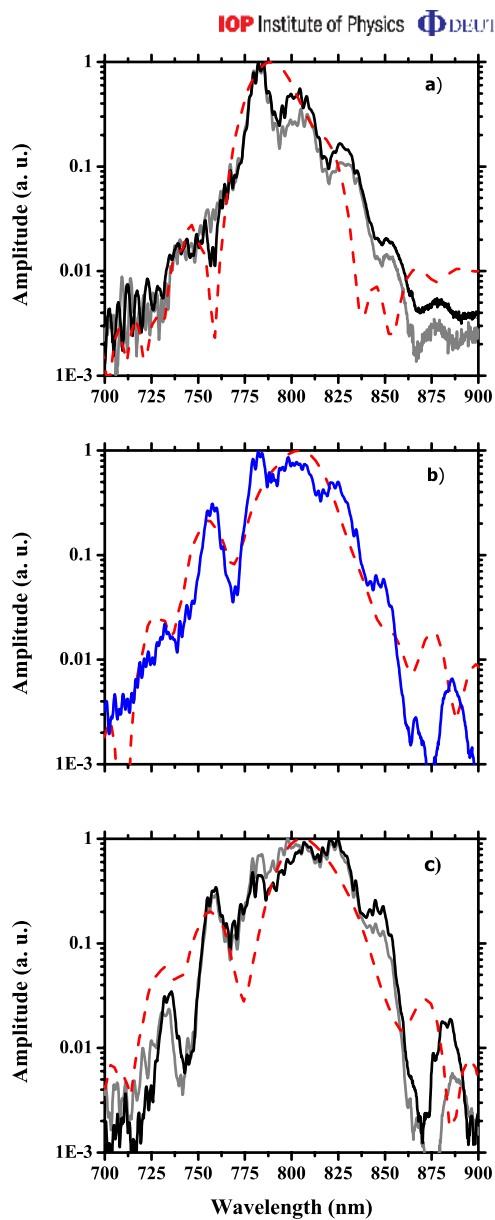
Figure 8. Laser pulse spectra for pulse energies 50 (a), 120 (b) and 150 mJ (c) measured in the experiment (solid lines are for different shots in (a) and (c) and the average of 4 shots is shown in (b)) and obtained in simulations (dashed lines). Parameters are indicated in the text.
