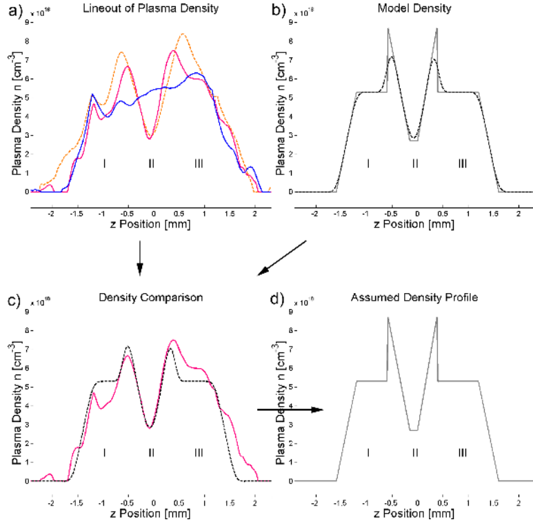
Figure 5.3. a) Measured plasma densities along the laser axis of the undisturbed jet (blue line), after the introduction of a 50 \mu\text{m} diameter wire (dashed amber line) and a 25 \mu\text{m} wire (solid magenta line), \approx 500 \mu\text{m} below the axis. Note the decreased length at FWHM of the density-diluted region II, which is \approx 440 \mu\text{m} with the 25 \mu\text{m} wire and \approx 610 \mu\text{m} with the 50 \mu\text{m} wire. All interferograms were recorded using \text{H}_2 at 9 bar backing pressure and a 3 mm supersonic nozzle. b) Broken line model density (grey solid line), motivated by simulations [63]. Subjecting this theoretical density distribution to a blur corresponding to the experimental resolution limitations in the measurements, provides an apparent density as depicted by the black dashed curve. c) Comparison between blurred model density and measured density for the 25 \mu\text{m} wire. d) shows the density used as input data for the PIC simulations, presented in Paper V.
