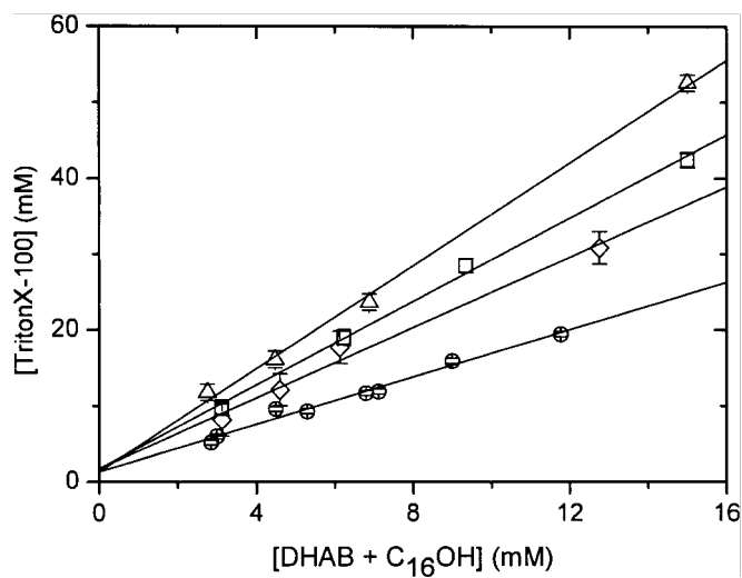
Figure 4A. R_{sol} relationships between [TritonX-100] vs. [DHAB + C 16 OH]: (○) 0 mol% C 16 OH (◇) 15 mol% C 16 OH (□) 25 mol% C 16 OH (Δ) 34 mol% C 16 OH.
