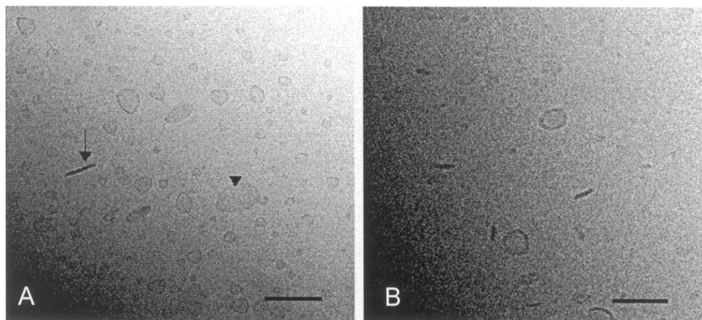
Figure 7. DHAB bilayers containing 0 mol% C_{10}OH (A) and 30 mol% C_{10}OH (B). The size of the bar represents 100 nm.
