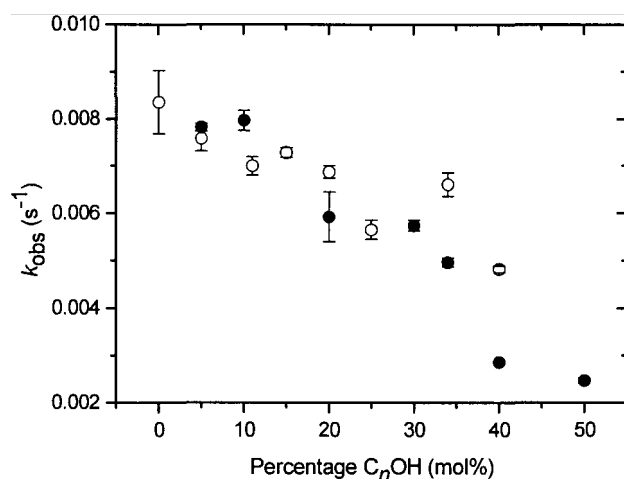
Figure 2. First-order rate constants for the decarboxylation of 1 embedded in DHAB vesicles containing C 10 OH (●) and C 16 OH (○). Error bars denote the standard deviation of at least 5 independent measurements.
