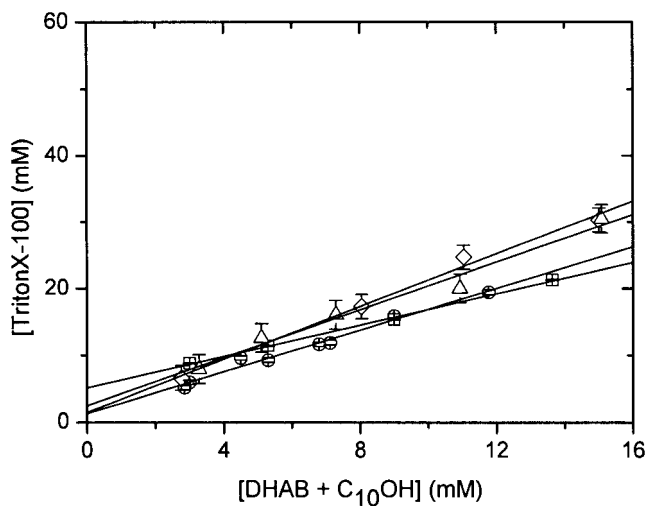
Figure 4B. R_{sol} relationships between [TritonX-100] vs. [DHAB + C 10 OH]: (○) 0 mol% C 10 OH (◇) 20 mol% C 10 OH (□) 34 mol% C 10 OH (Δ) 50 mol% C 10 OH.
