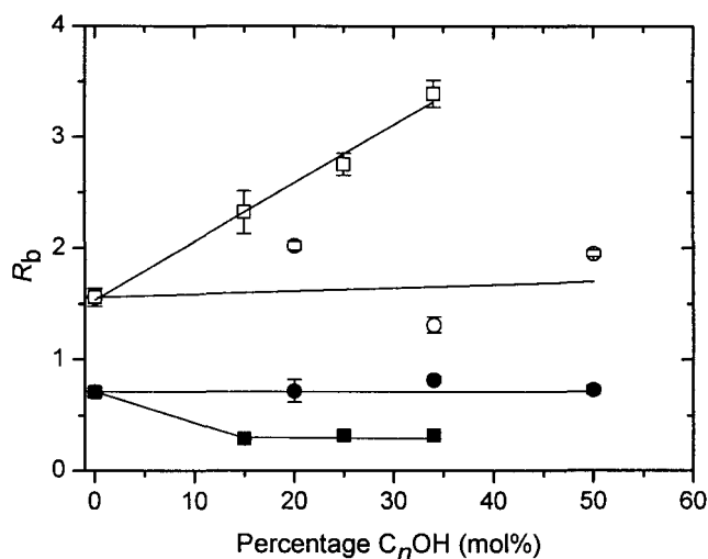
Figure 5. Slopes of Figure 3 and 4 vs. percentage of C_n OH in the DHAB mixtures: ( \square ) 0 mol% R_{sol} C_{16} OH; ( \blacksquare ) R_{sat} C_{16} OH; ( \circ ) R_{sol} C_{10} OH; ( \bullet ) R_{sat} C_{10} OH. Lines are drawn to guide the eye
