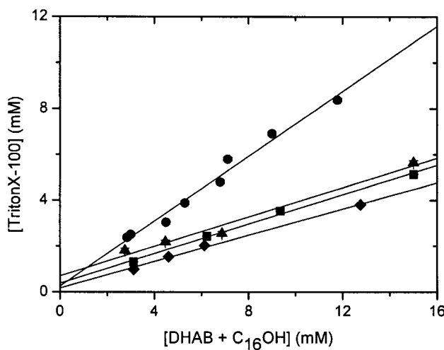
Figure 3A. R_{\text{sat}} relationships between [TritonX-100] vs. [DHAB + C 16 OH]: (●) 0 mol% C 16 OH (◆) 15 mol% C 16 OH (■) 25 mol% C 16 OH (▲) 34 mol% C 16 OH.
