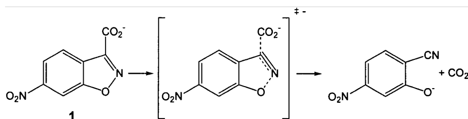
Scheme 1. Decarboxylation of 6-nitrobenzisoxazole-3-carboxylate anion (6-NBIC).
