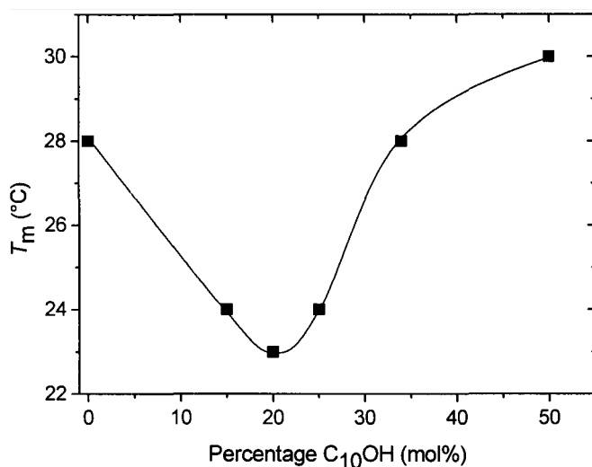
Figure 6. Relationship between T_m and the percentage of C_{10} OH (mol%) in DHAB/ C_{10} OH mixtures. The line is drawn to guide the eye.
