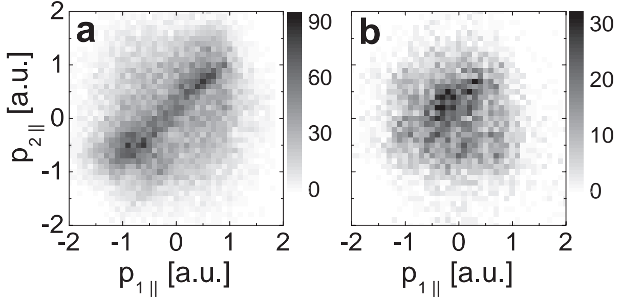
FIG. 2: The electron momentum correlation for the momentum components parallel to the light beam polarization vector: (a) \text{N}_2 at 1.5 \times 10^{14} \text{ W/cm}^2 and (b) \text{O}_2 at 1.7 \times 10^{14} \text{ W/cm}^2 .
