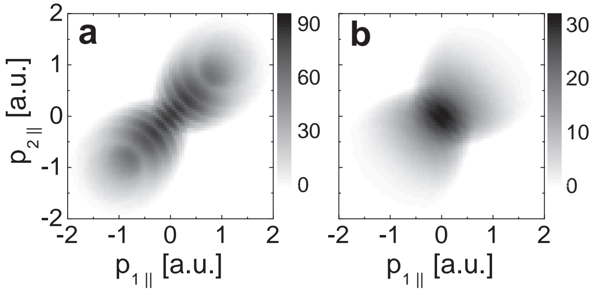
FIG. 3: Calculated electron momentum correlation for \text{N}_2 (a) and \text{O}_2 (b). The light intensities are chosen as in Fig. 2.
