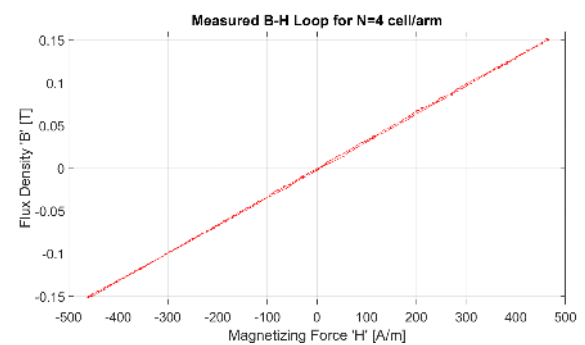
FIGURE 13. B-H loop obtained from measurement
