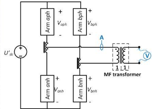
FIGURE 10. MMC module testbed with measurement circuit for N=2;4 cells/arm
