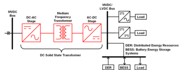
FIGURE 1. HV_IBDC as a DC grid building block
