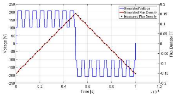
FIGURE 12. Measured and simulated flux densities
