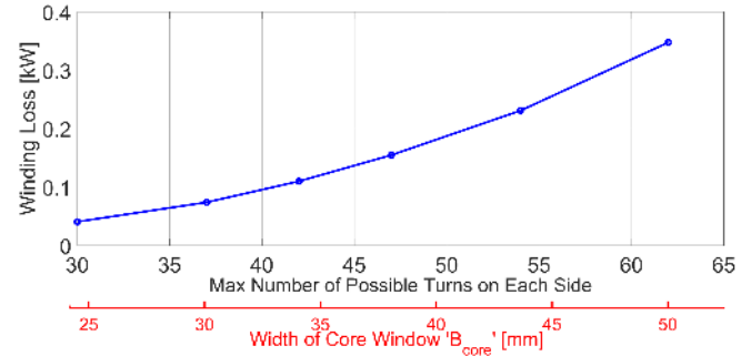
FIGURE 7. Calculated winding loss
