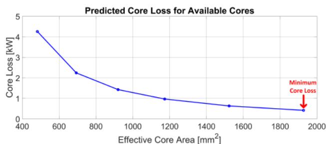
FIGURE 6. Core loss vs. core cross-section area
