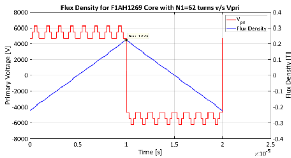
FIGURE 4. AC voltage vs. flux density
