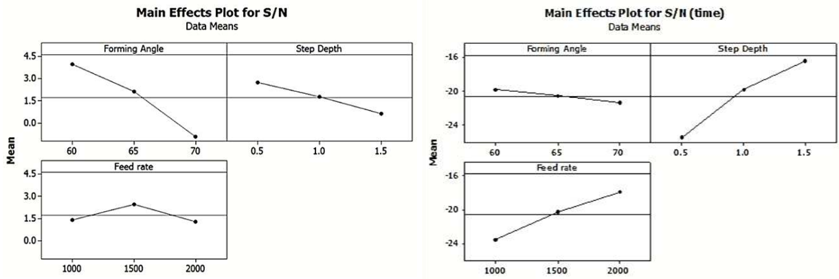
Figure 4. Response graph for surface roughness and forming time
