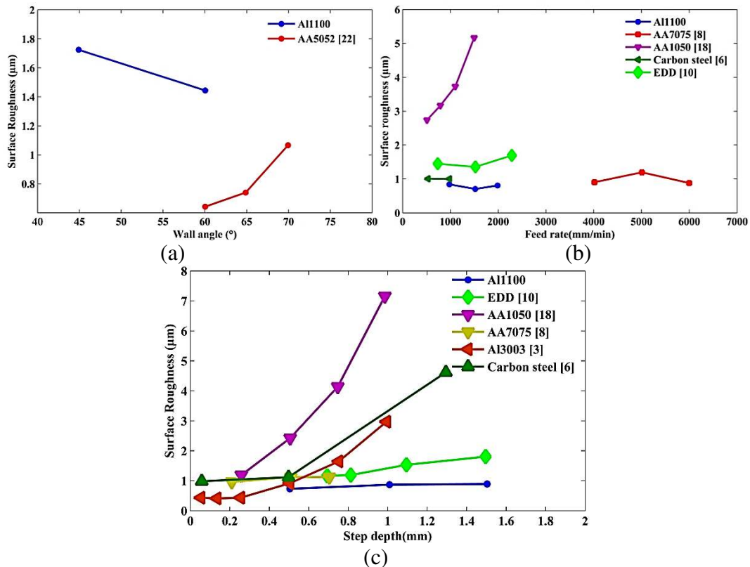
Figure 7. Effect of (a) wall thickness, (b) feed rate and (c) step depth on surface roughness
