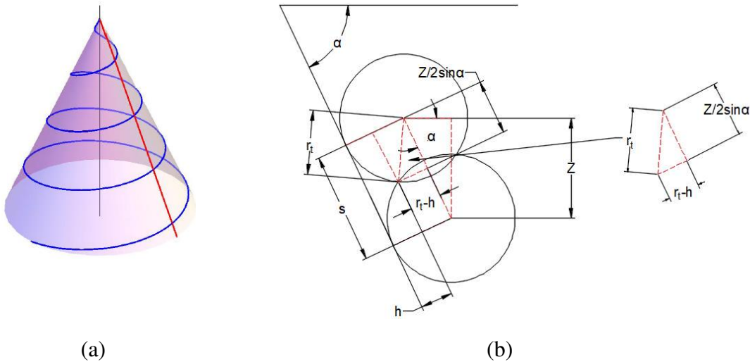
Figure 1. (a) The spiral tool path for the conical cup part and (b) the scallop height.
