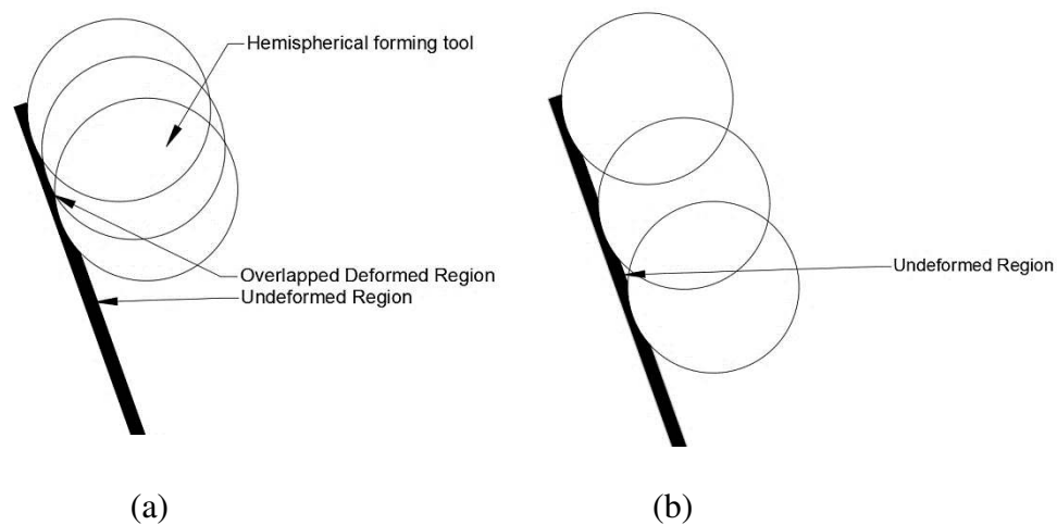
Figure 2. Deformation zone due to (a) small step depth and (b) larger step depth
