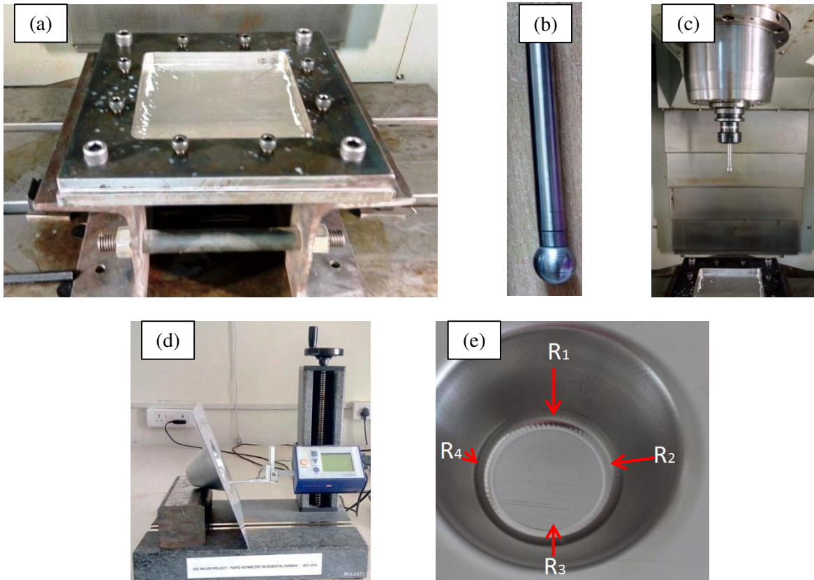
Figure 3. (a) Forming fixture, (b) forming tool, (c) the setup and (d) profilometer (e) direction of surface roughness measurement
