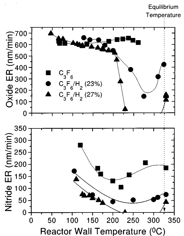
FIG. 11. (A) Oxide etch rates and (B) nitride etch rates as functions of wall temperature measured in C 3 F 6 (40 sccm), C 3 F 6 /H 2 (40 sccm/12 sccm), and C 3 F 6 /H 2 (40 sccm/15 sccm) discharges at 1400 W inductive power and 6 mTorr operating pressure at a RF bias power of 200 W (i.e., -100 V self-bias).
