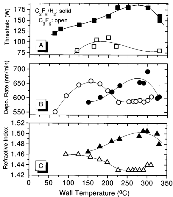
FIG. 10. (A) Threshold RF bias power for etching, (B) passive fluorocarbon deposition rate, and (C) the fluorocarbon refractive index as a function of reactor wall temperature in a C 3 F 6 (40 sccm) and a C 3 F 6 /H 2 (40 sccm/12 sccm) plasma at 1400 W inductive power and 6 mTorr operating pressure.
