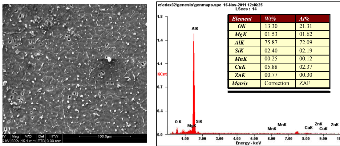
Figure 1. The SEM micrograph and EDX spectra of Al-4% Cu-2.5% Mg/5 wt% Al 2 O 3 .
